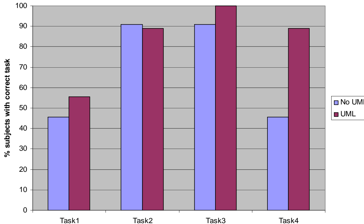
Task Correctness
