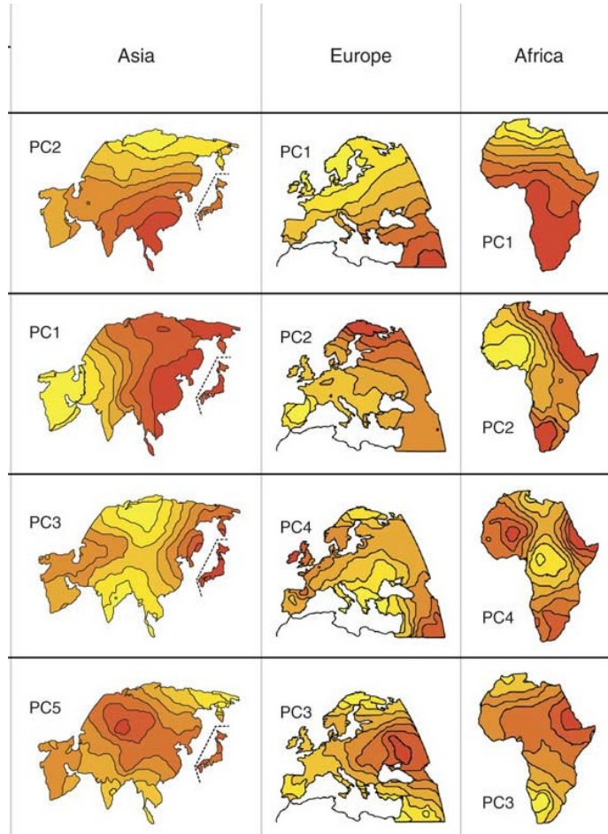
Figure 17.3: Principal components of genetic variation in the old world, according to Cavalli-Sforza et al. (1994), as re-drawn by Novembre and Stephens (2008).
