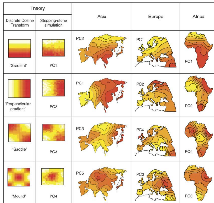
Figure 17.4: How the PCA patterns can arise as numerical artifacts (far left column) or through simple genetic diffusion (next column). From Novembre and Stephens (2008).
