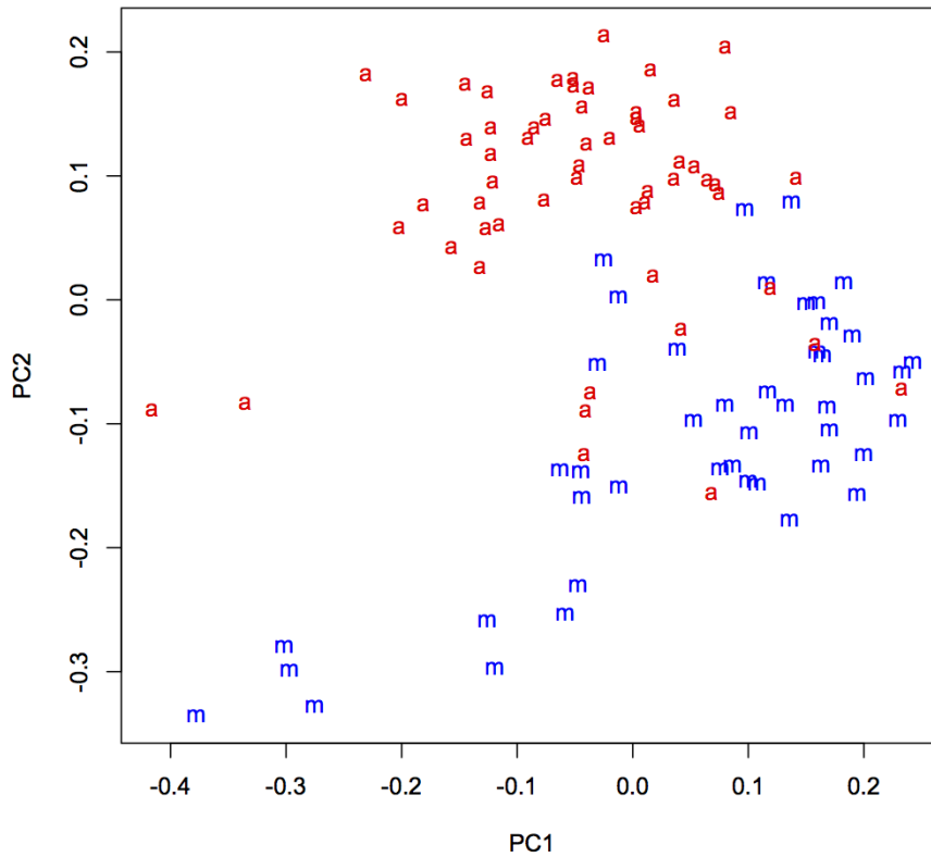
Figure 17.2: Projection of the Times stories on to the first two principal components. Labels: “a” for art stories, “m” for music.
