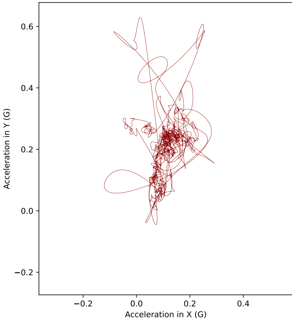
A1 acceleration in XY plane (Top view)
