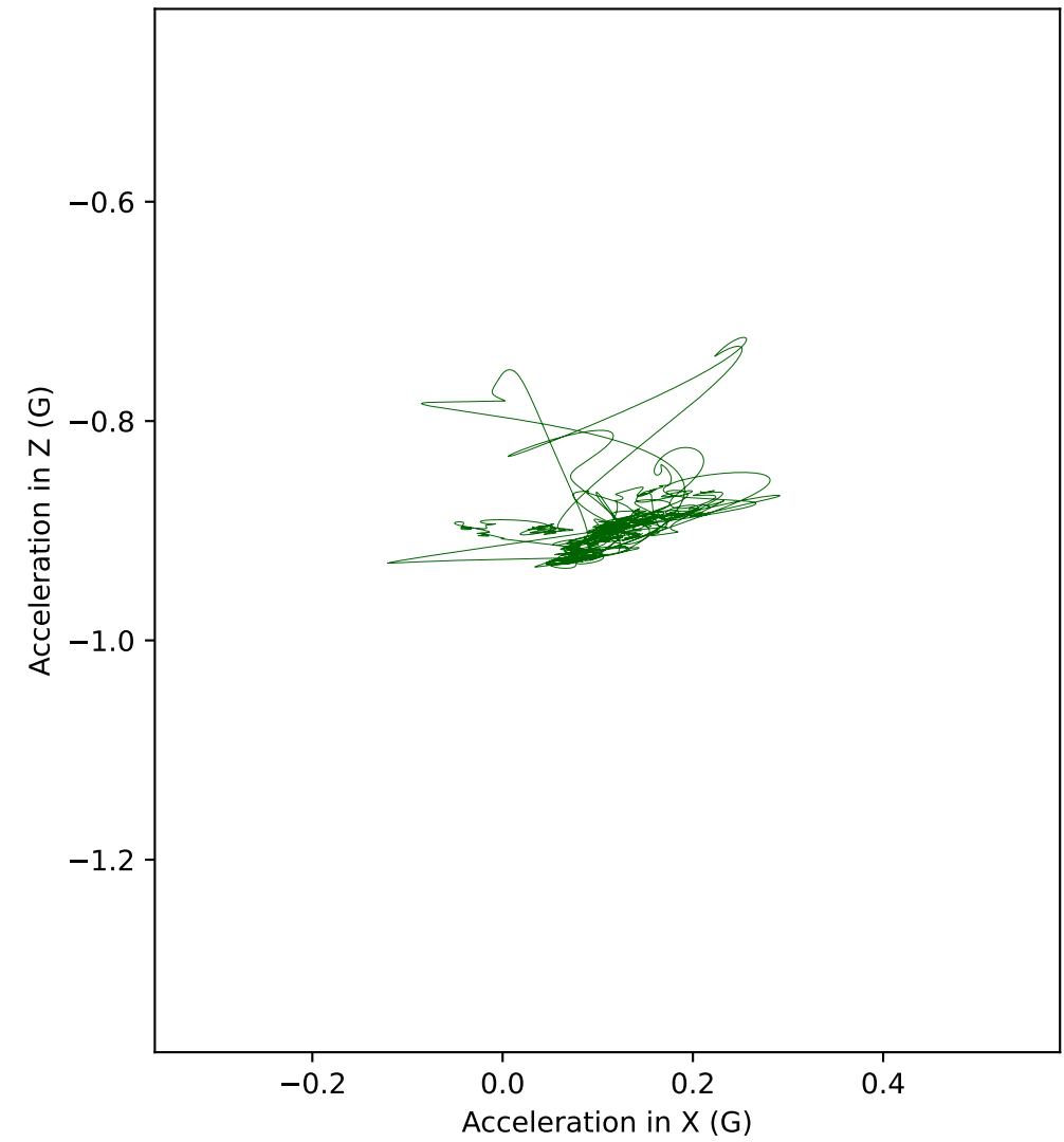
A1 acceleration in XZ plane (Front view)
