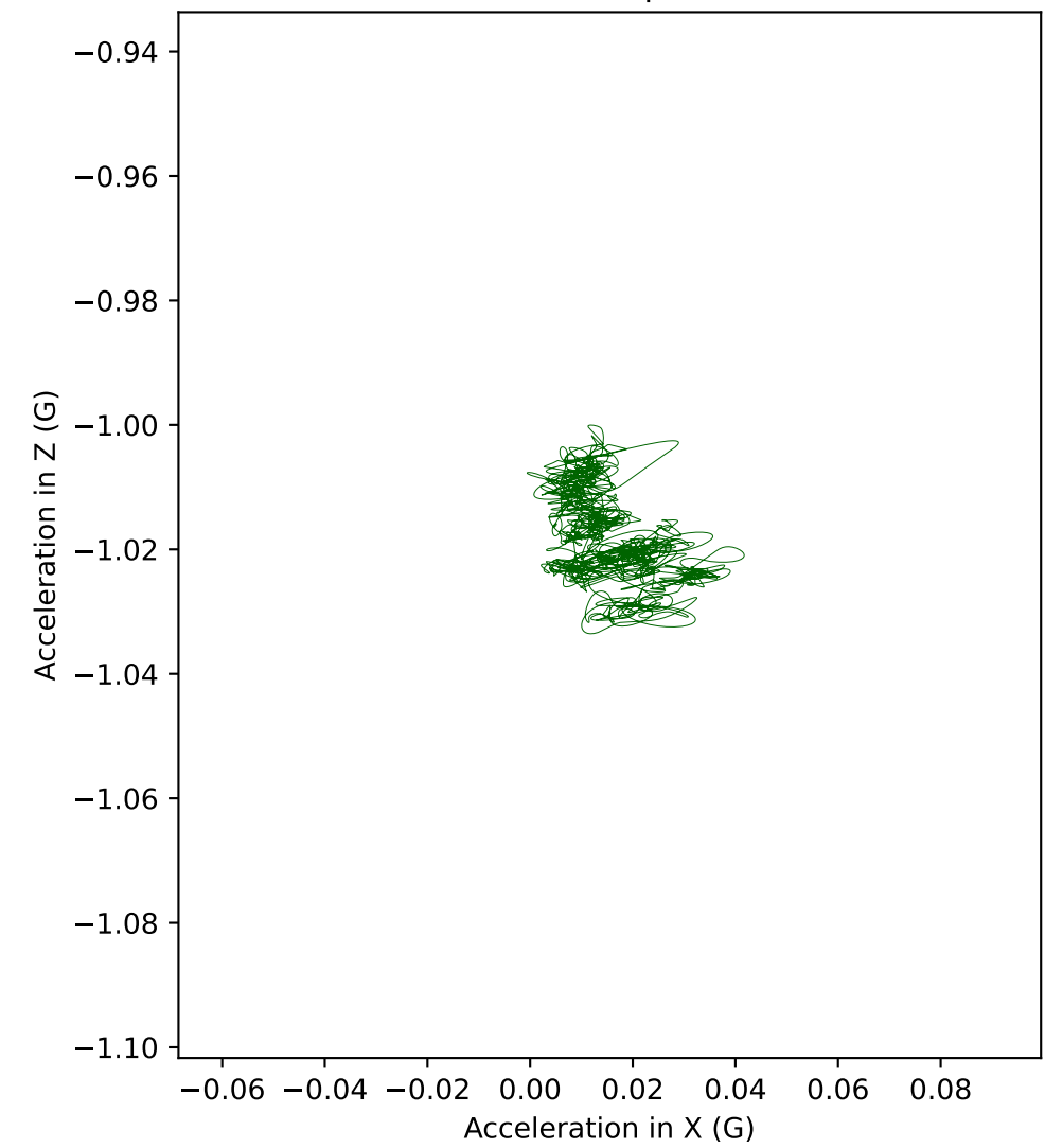
A2 acceleration in XZ plane (Front view)
