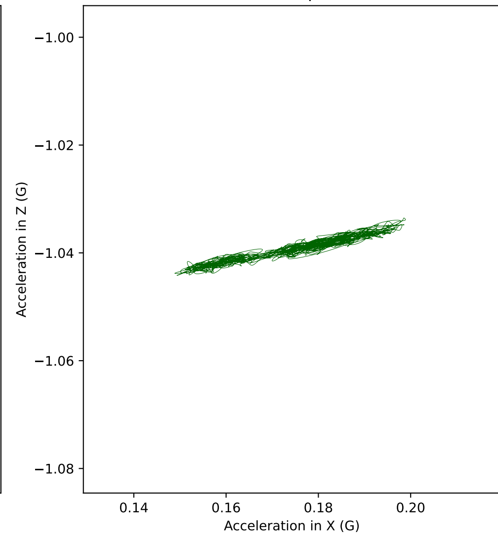
A3 acceleration in XZ plane (Front view)
