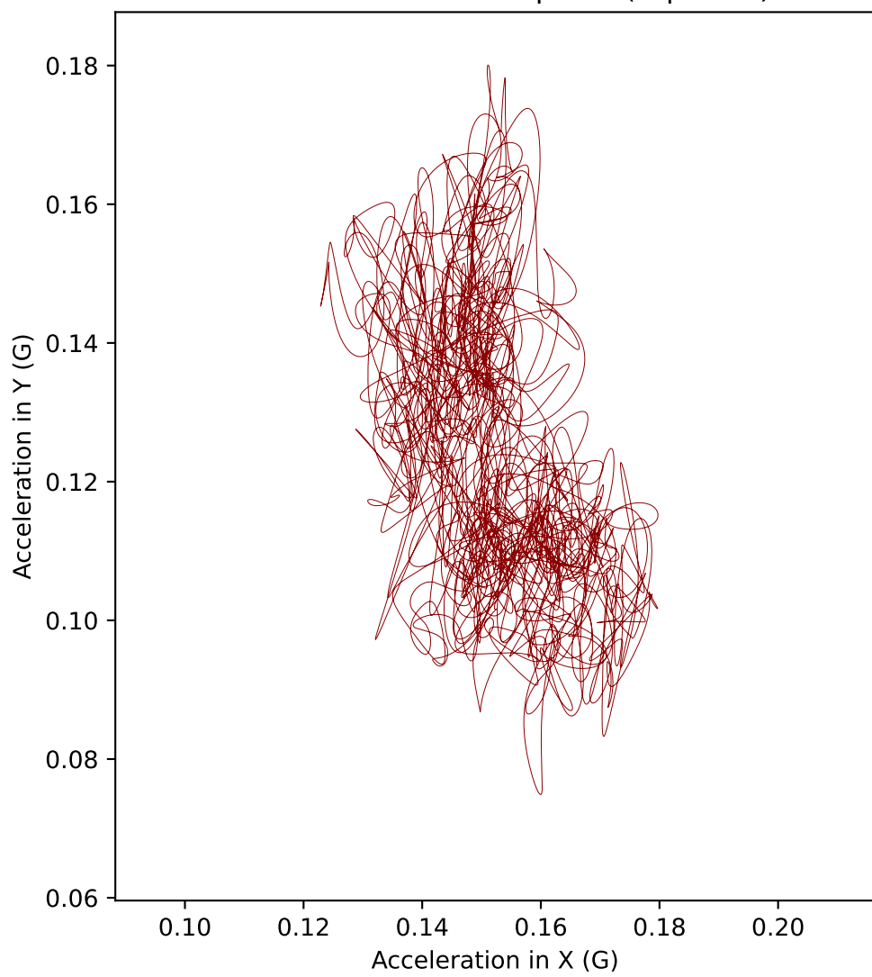
A4 acceleration in XY plane (Top view)
