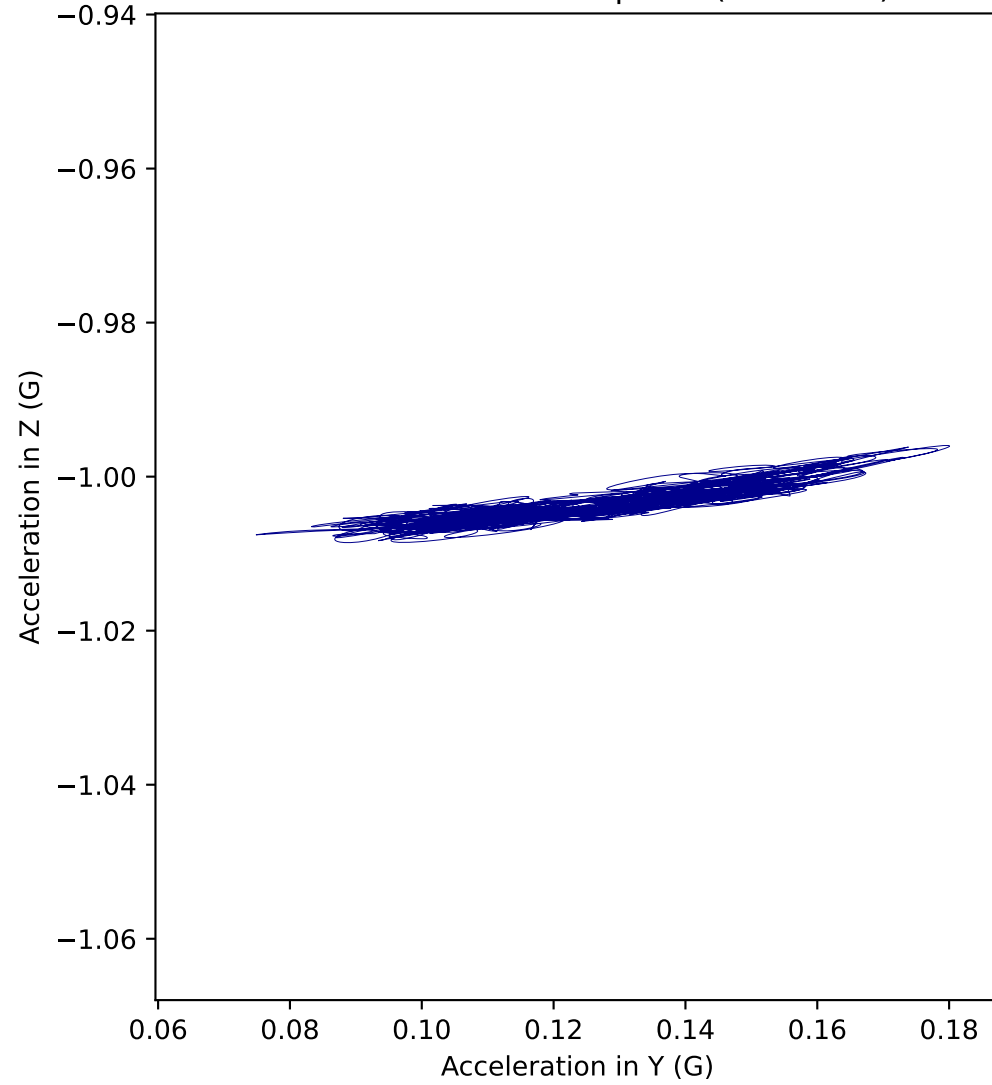
A4 acceleration in YZ plane (Side view)
