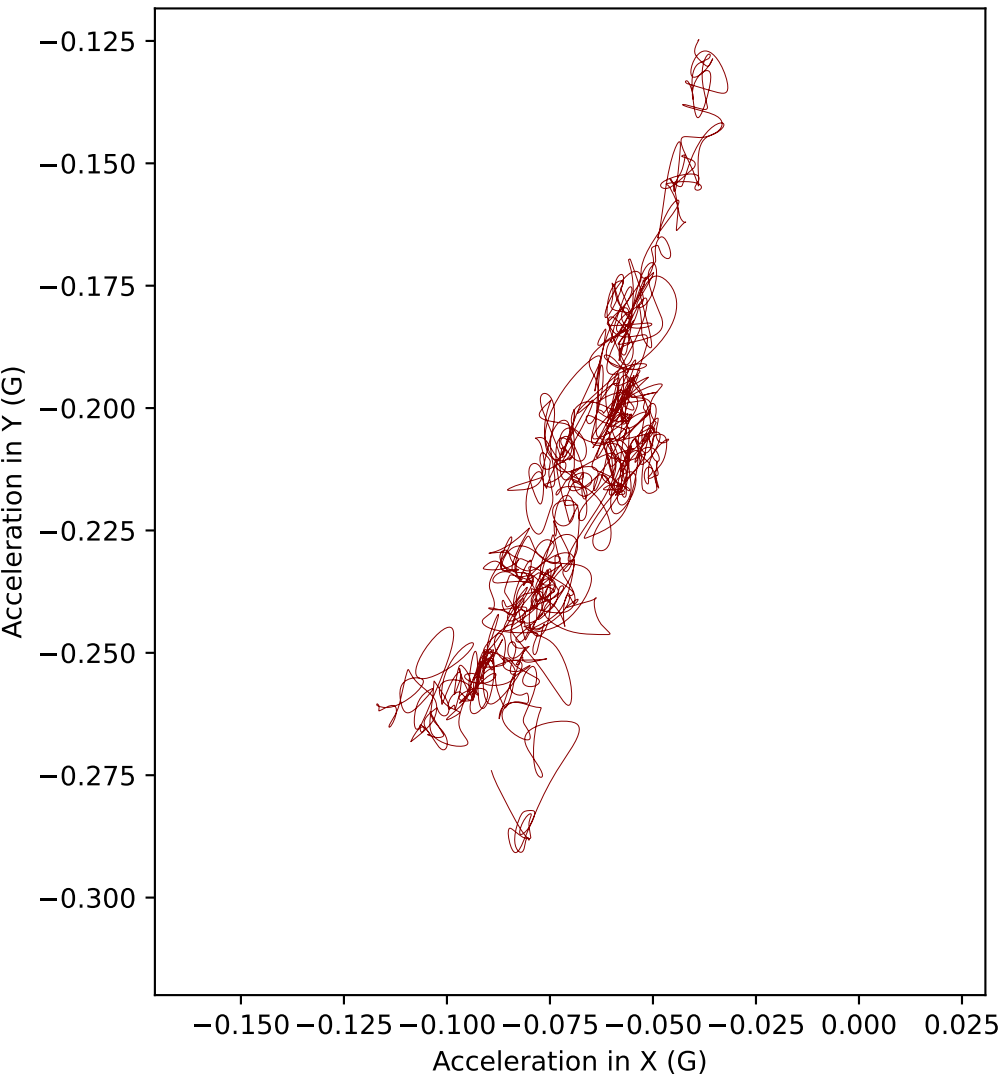
A5 acceleration in XY plane (Top view)
