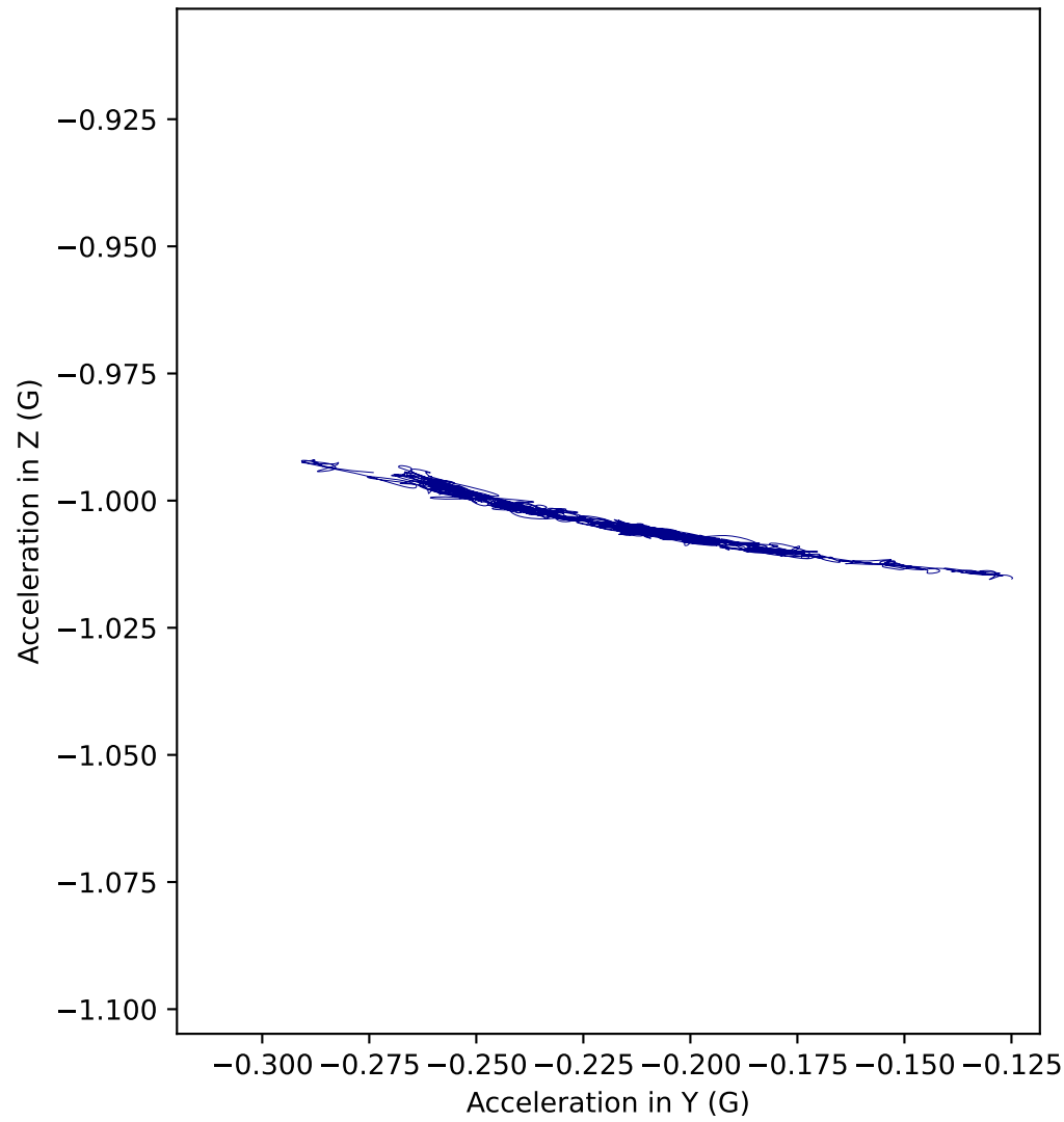
A5 acceleration in YZ plane (Side view)
