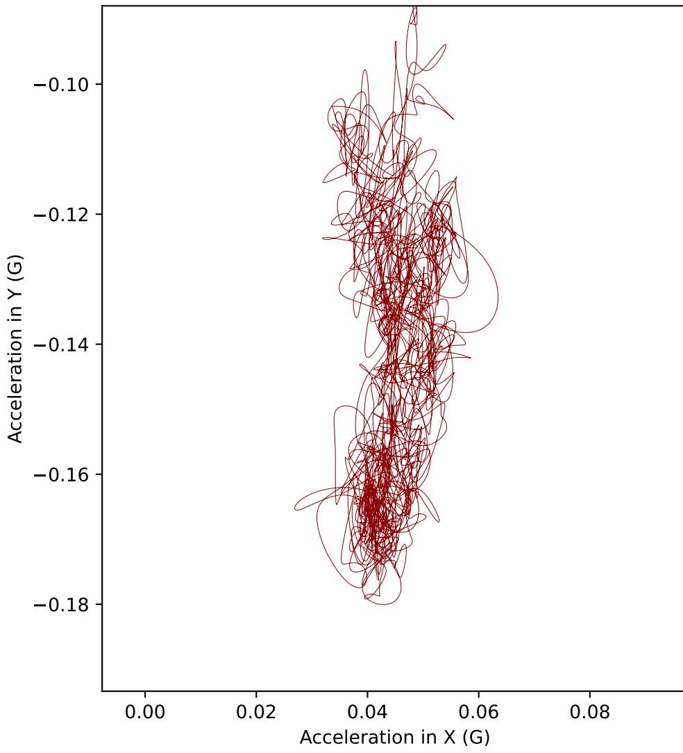
A6 acceleration in XY plane (Top view)
