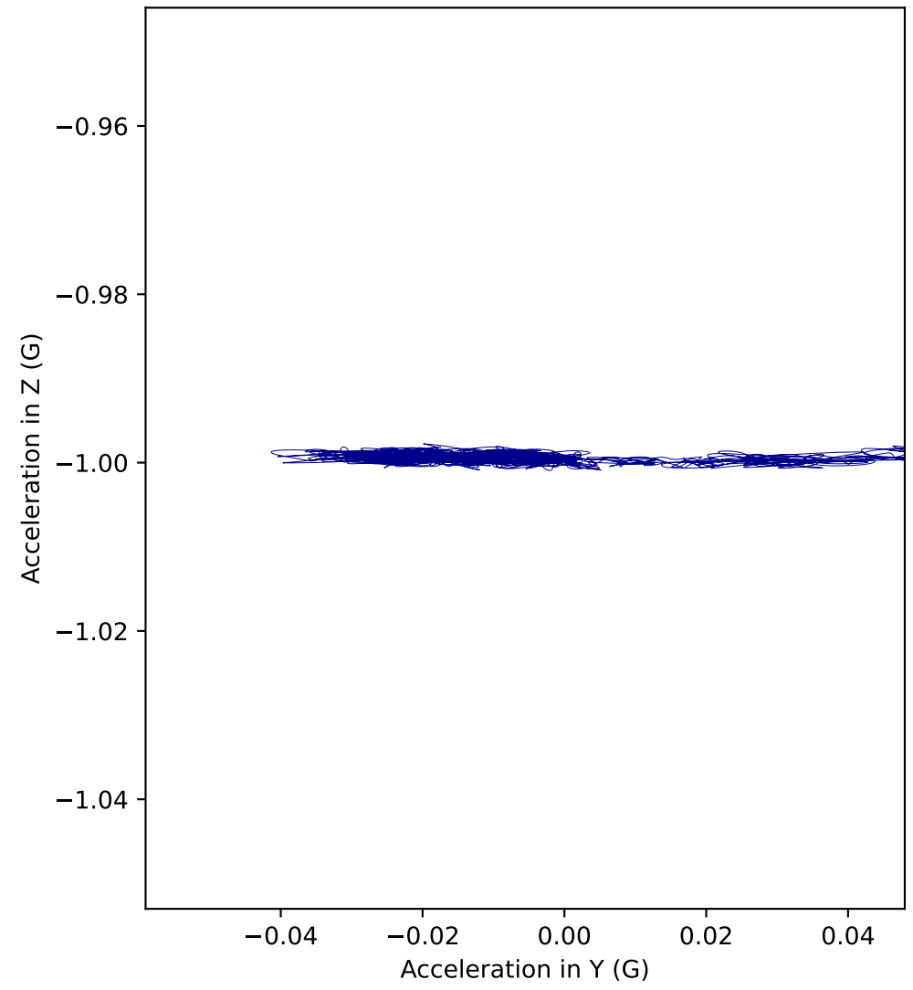
A8 acceleration in YZ plane (Side view)
