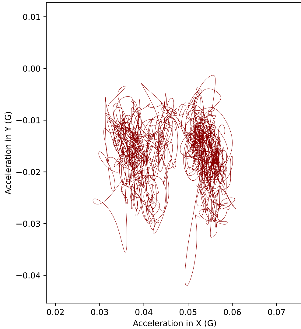
B1 acceleration in XY plane (Top view)
