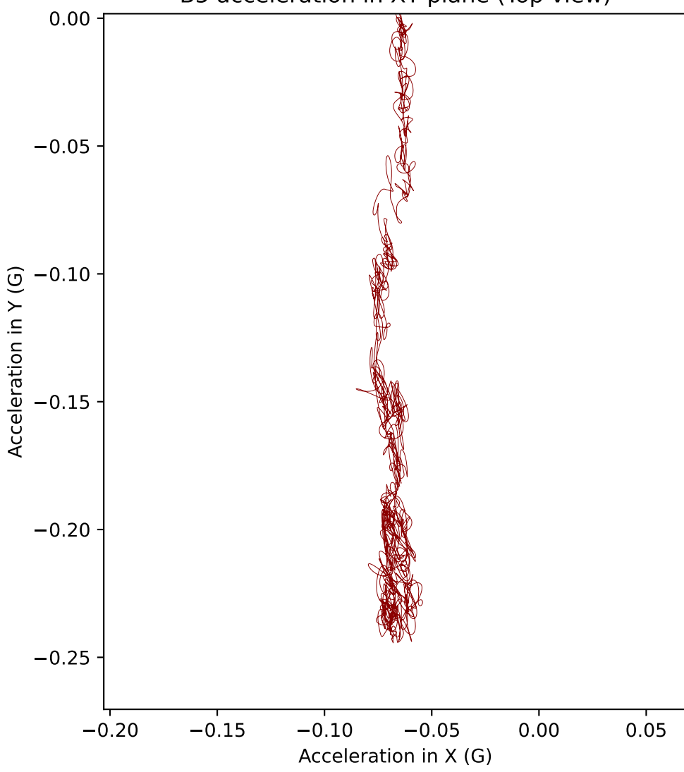
B5 acceleration in XY plane (Top view)
