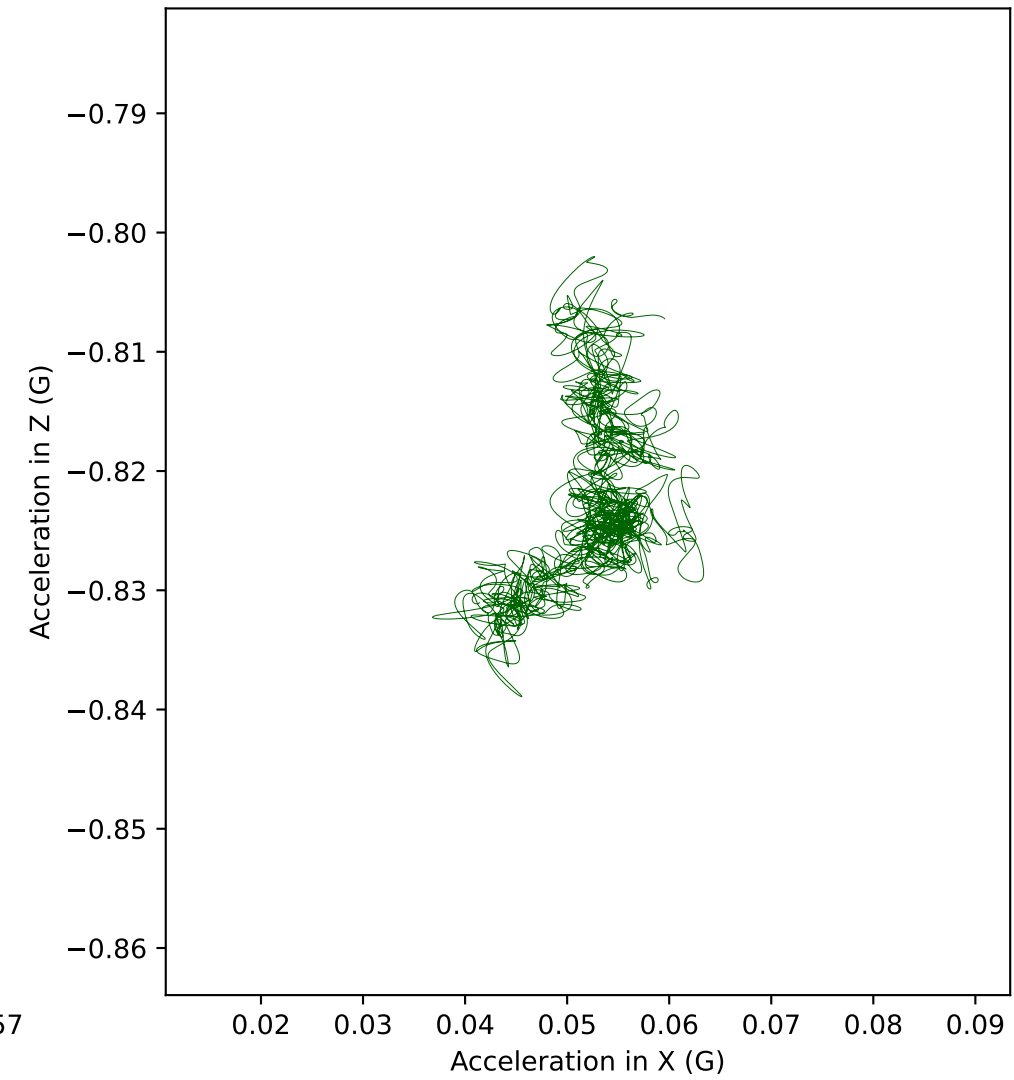
B6 acceleration in XZ plane (Front view)
