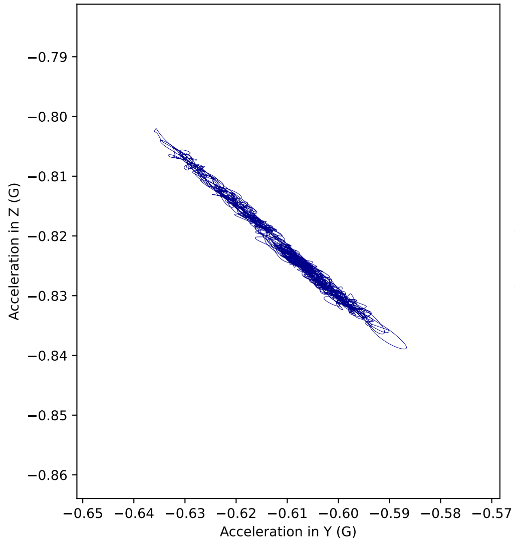
B6 acceleration in YZ plane (Side view)
