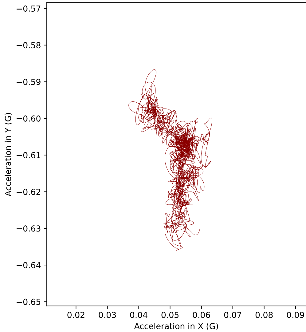
B6 acceleration in XY plane (Top view)
