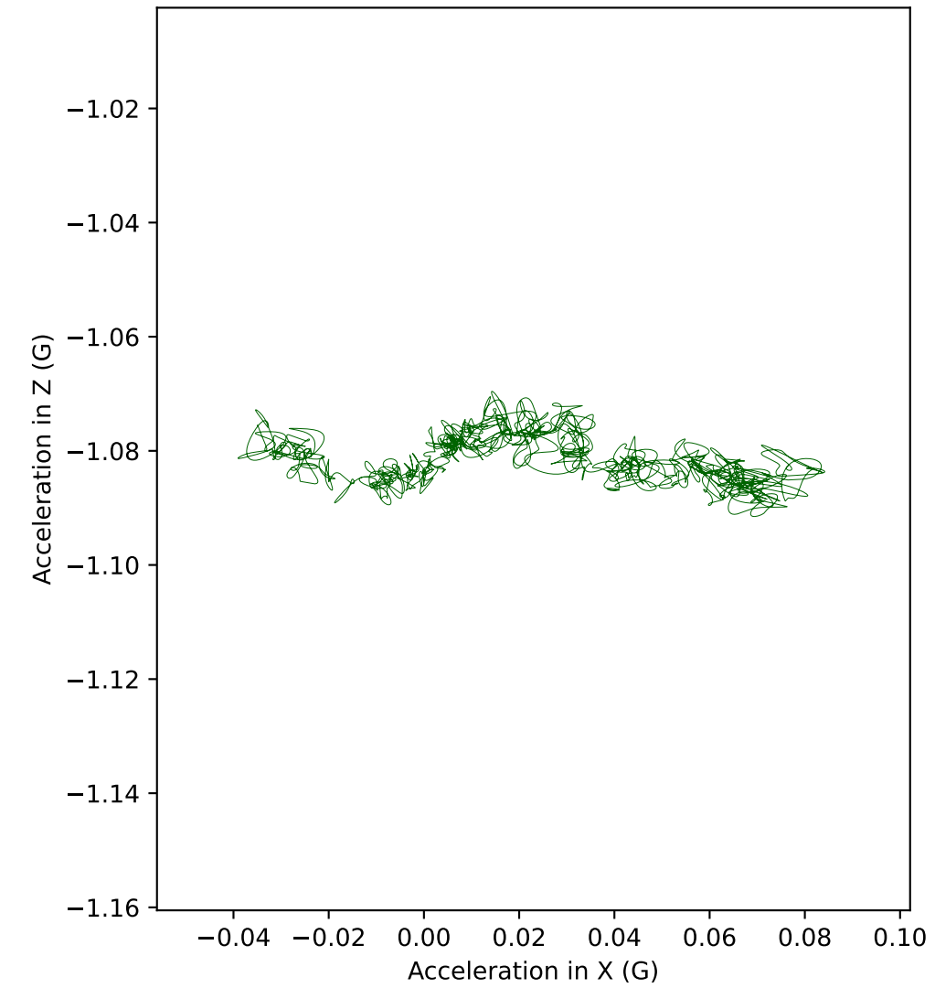
B7 acceleration in XZ plane (Front view)
