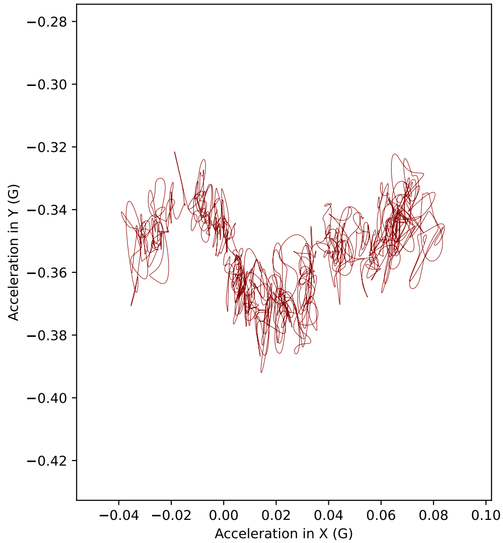
B7 acceleration in XY plane (Top view)
