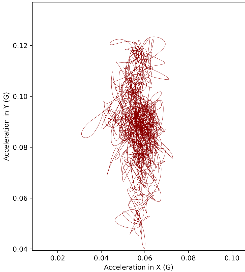
C1 acceleration in XY plane (Top view)
