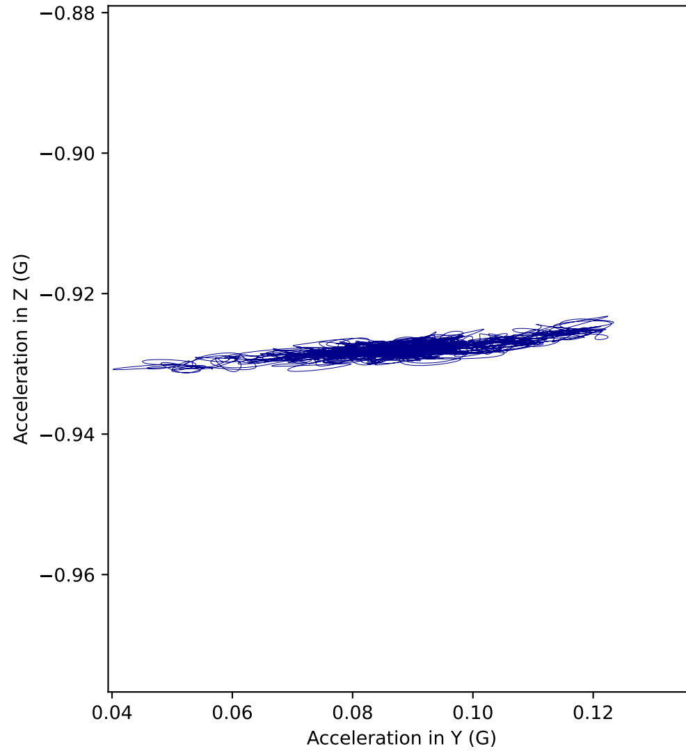
C1 acceleration in YZ plane (Side view)
