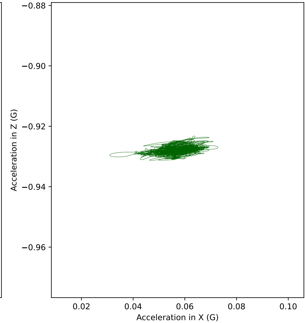
C1 acceleration in XZ plane (Front view)
