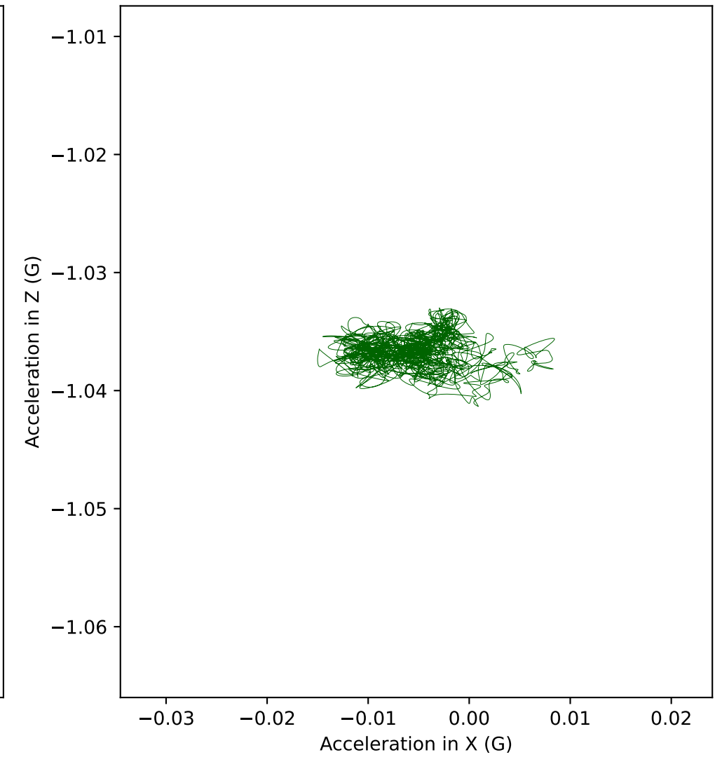
C3 acceleration in XZ plane (Front view)
