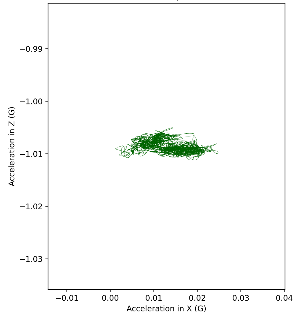
C5 acceleration in XZ plane (Front view)
