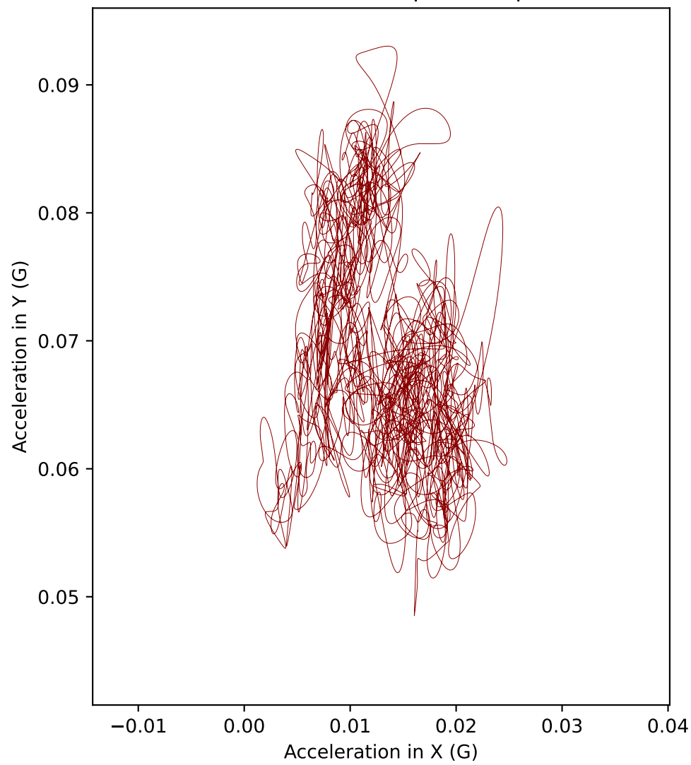
C5 acceleration in XY plane (Top view)
