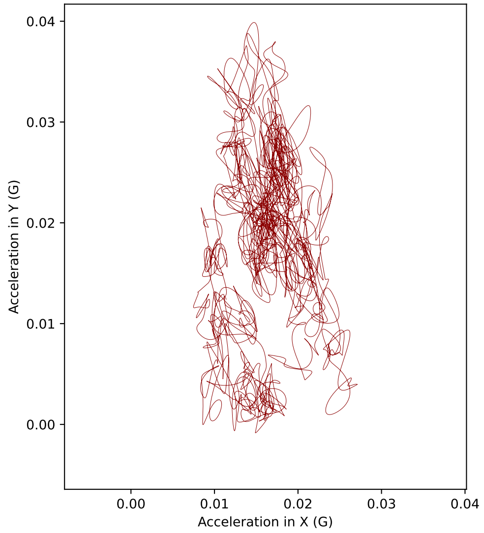
C6 acceleration in XY plane (Top view)
