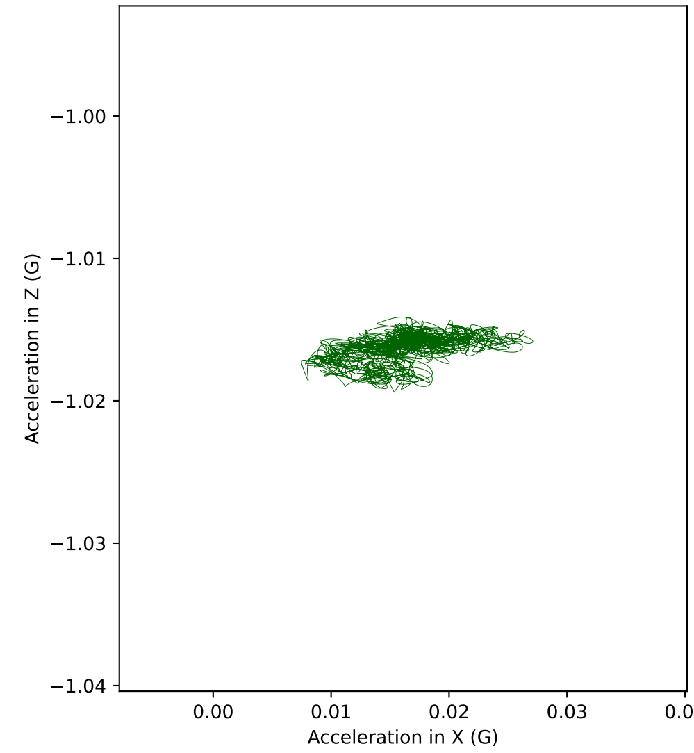
C6 acceleration in XZ plane (Front view)
