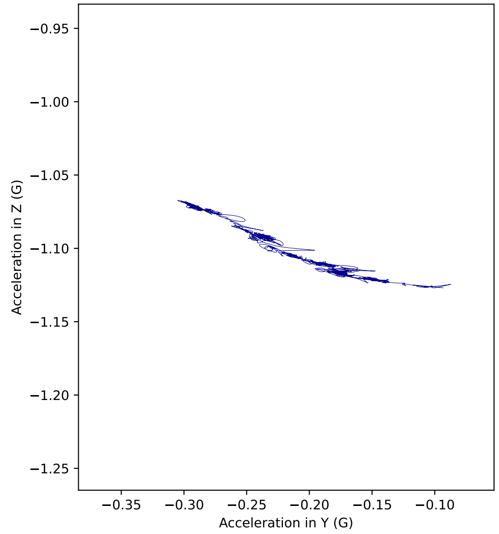
C7 acceleration in YZ plane (Side view)
