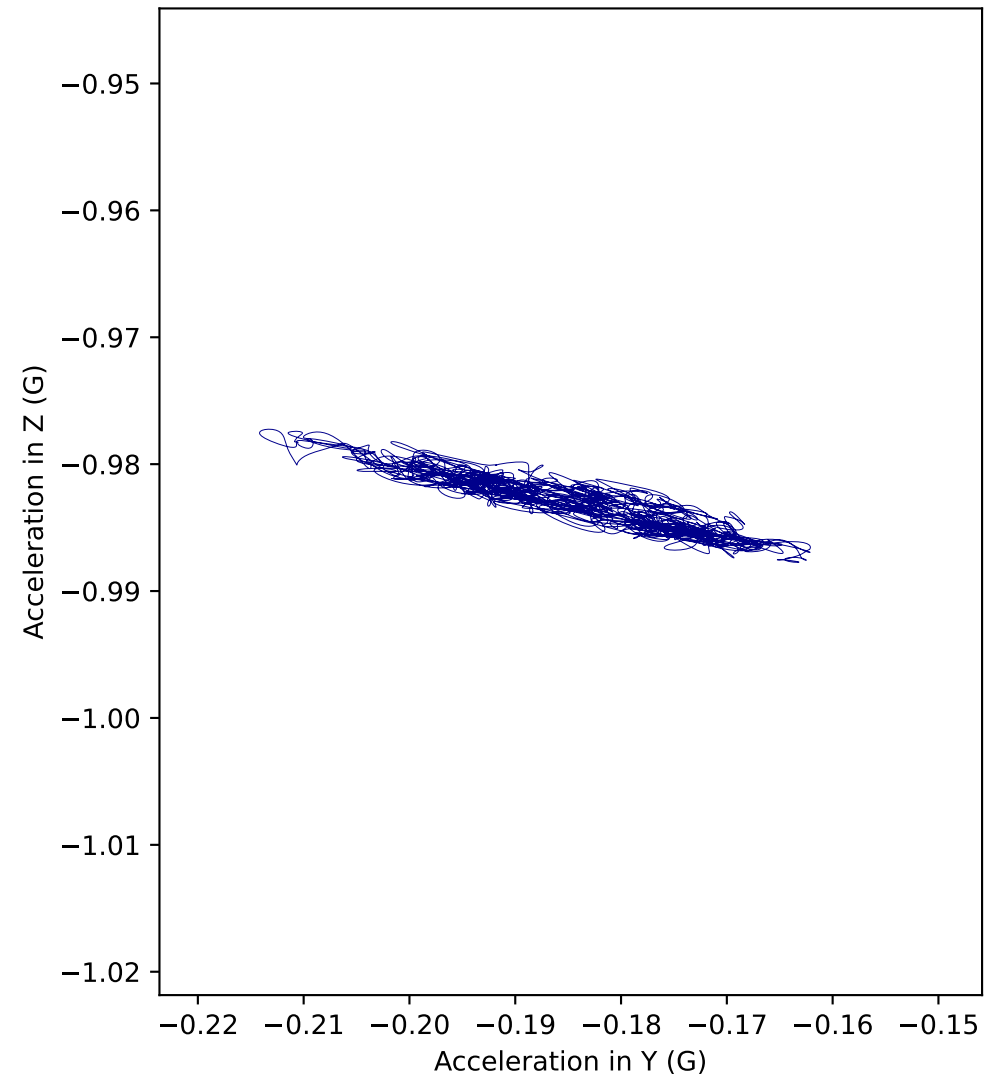
C8 acceleration in YZ plane (Side view)
