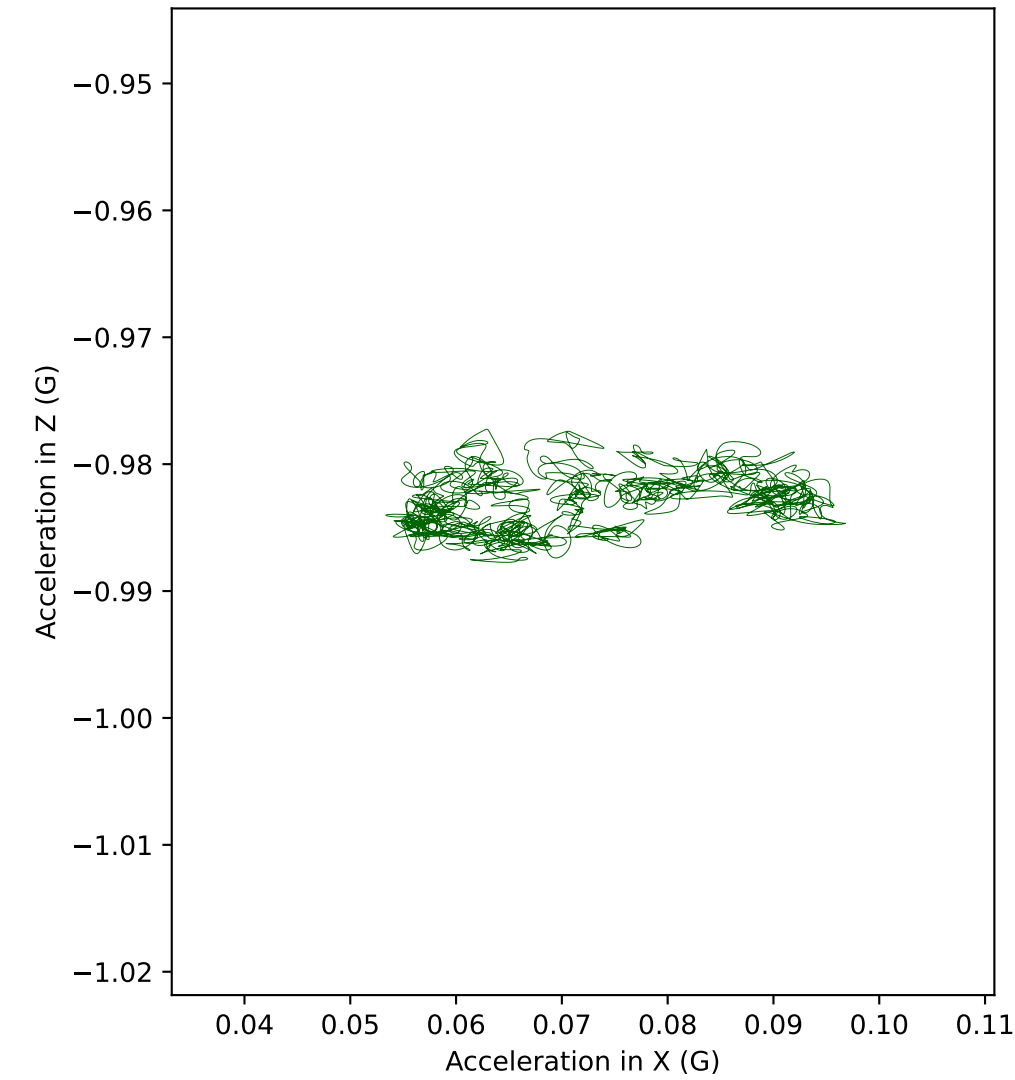
C8 acceleration in XZ plane (Front view)
