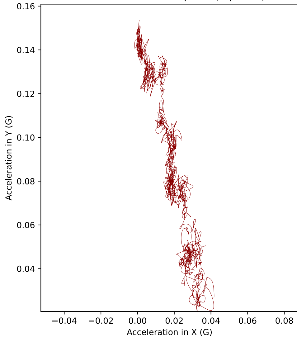
D3 acceleration in XY plane (Top view)
