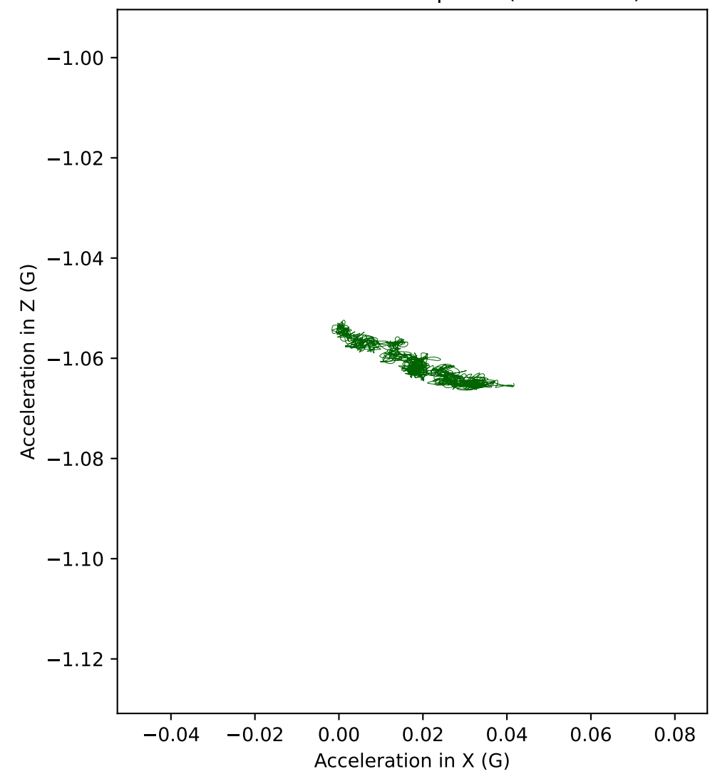
D3 acceleration in XZ plane (Front view)
