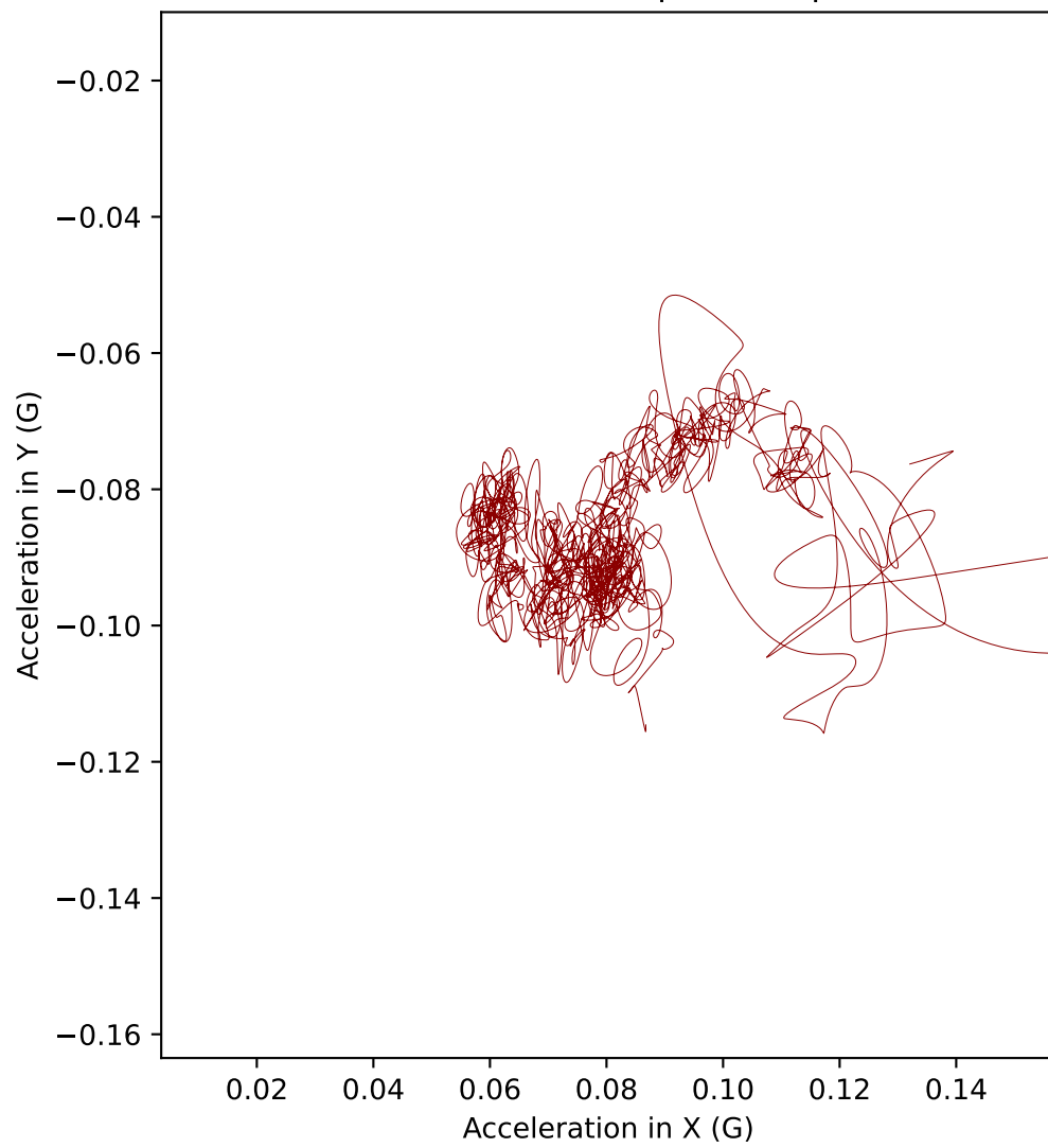
D4 acceleration in XY plane (Top view)
