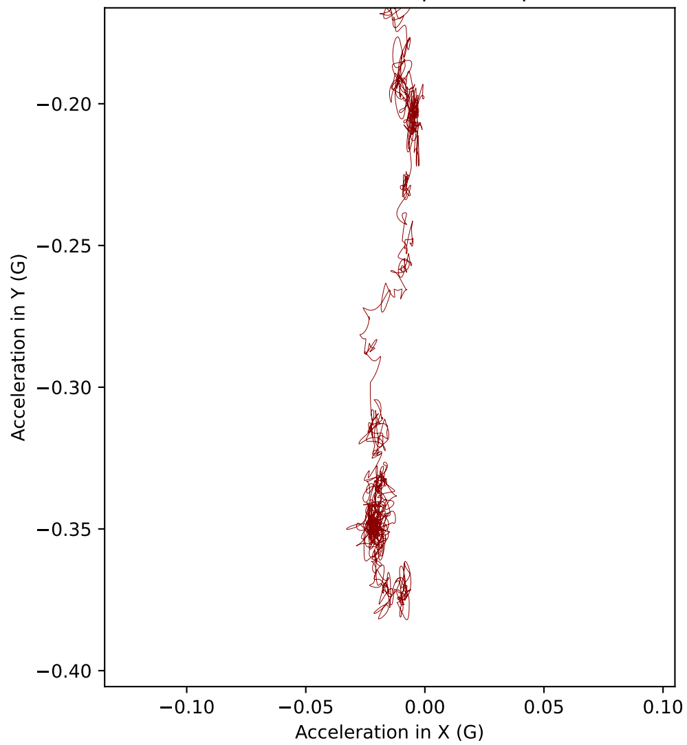
D5 acceleration in XY plane (Top view)
