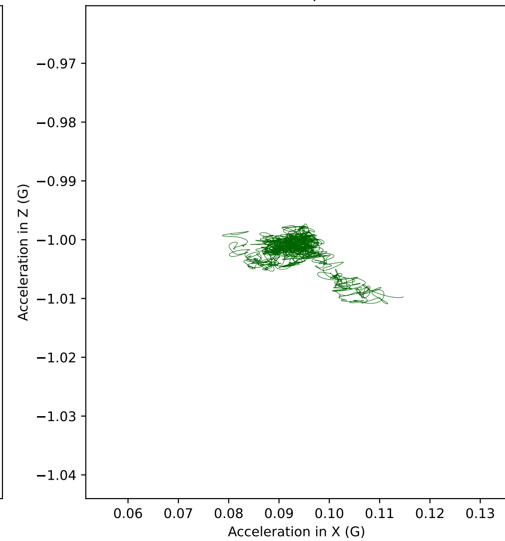
E4 acceleration in XZ plane (Front view)
