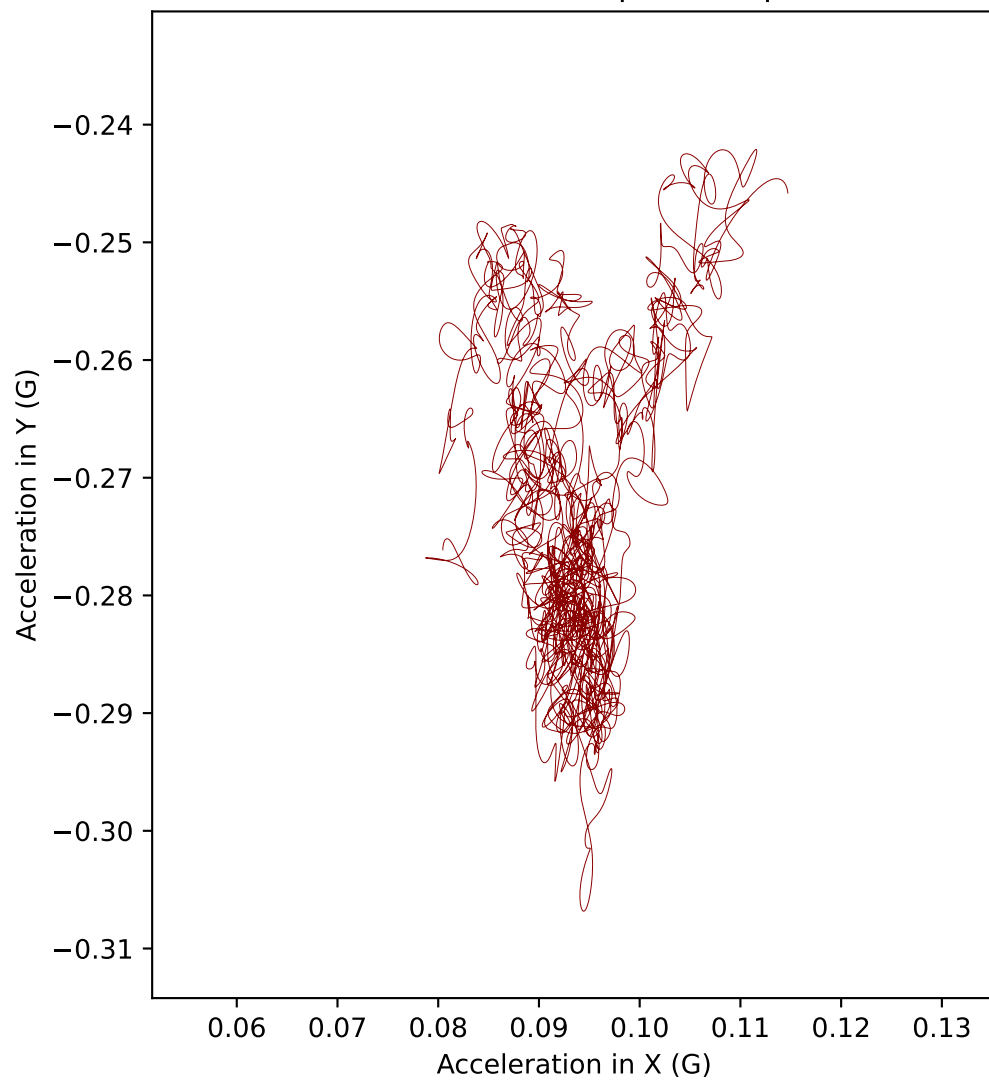
E4 acceleration in XY plane (Top view)
