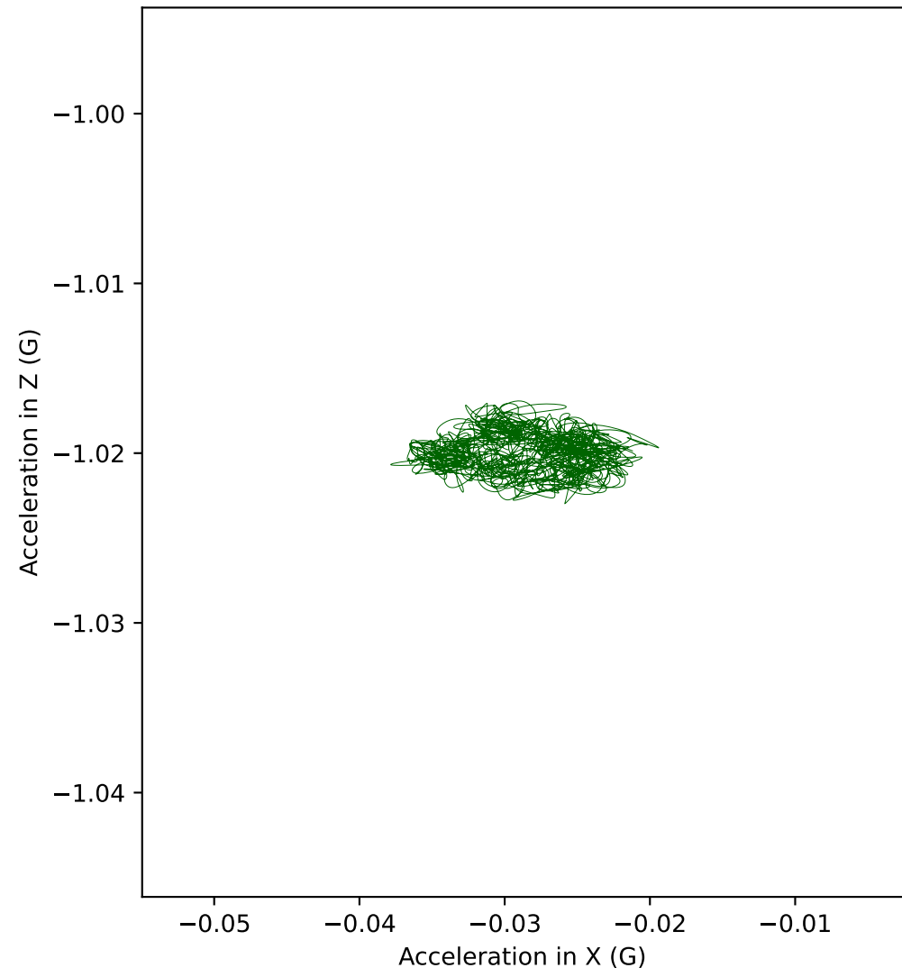
E5 acceleration in XZ plane (Front view)
