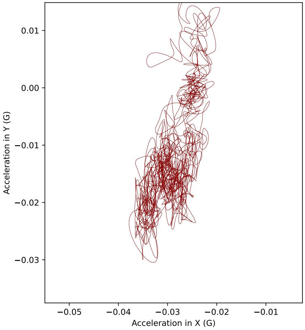
E5 acceleration in XY plane (Top view)
