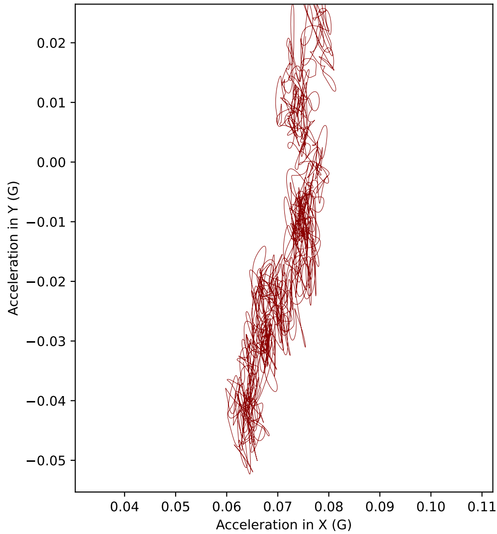
F1 acceleration in XY plane (Top view)
