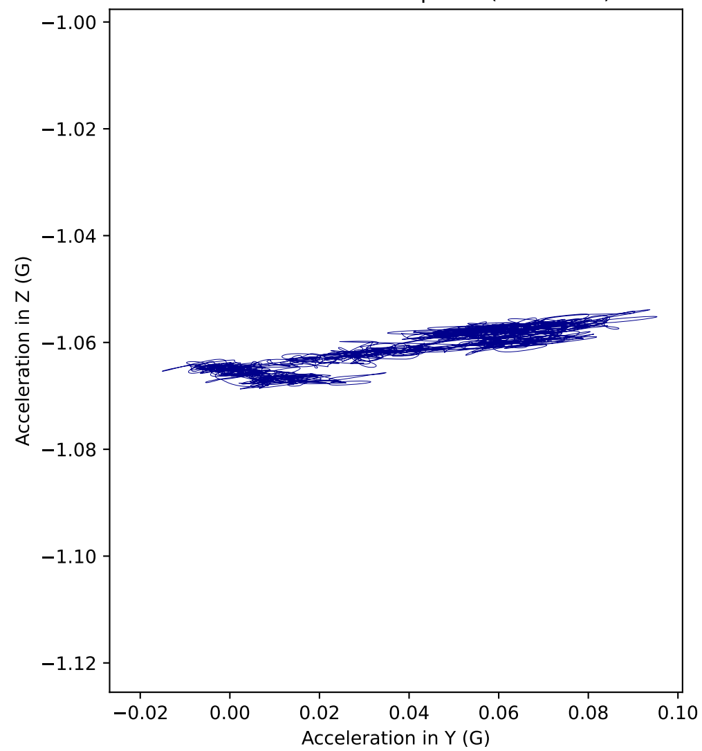
F3 acceleration in YZ plane (Side view)
