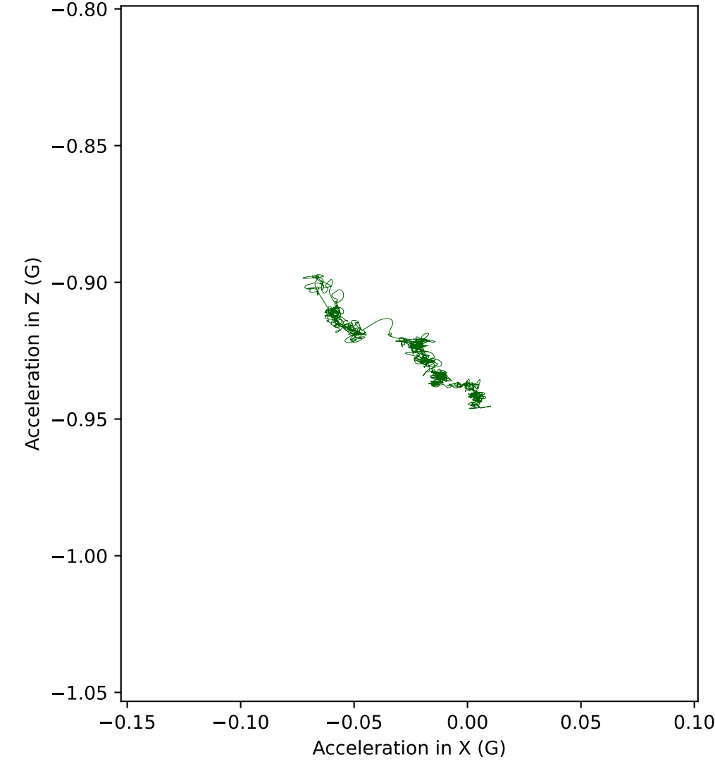
G1 acceleration in XZ plane (Front view)
