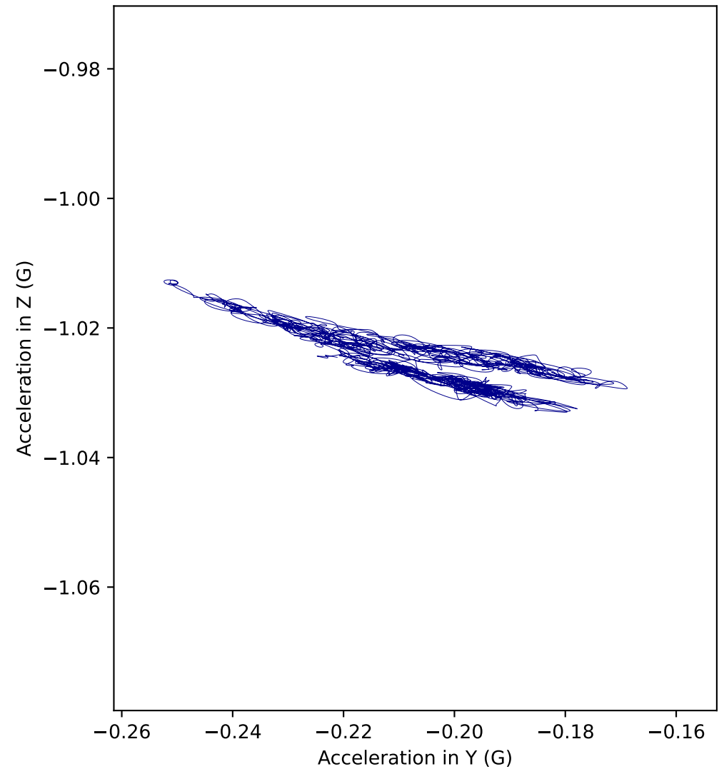
G2 acceleration in YZ plane (Side view)
