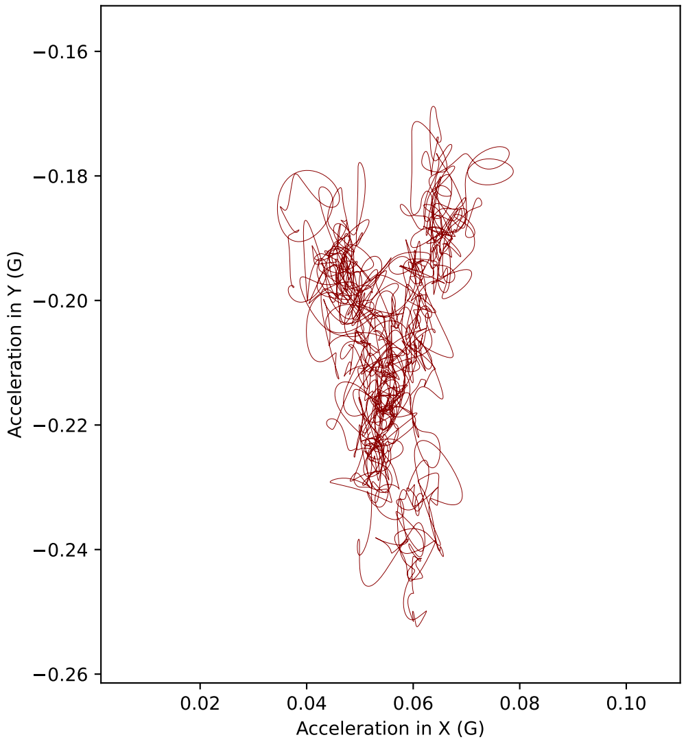
G2 acceleration in XY plane (Top view)
