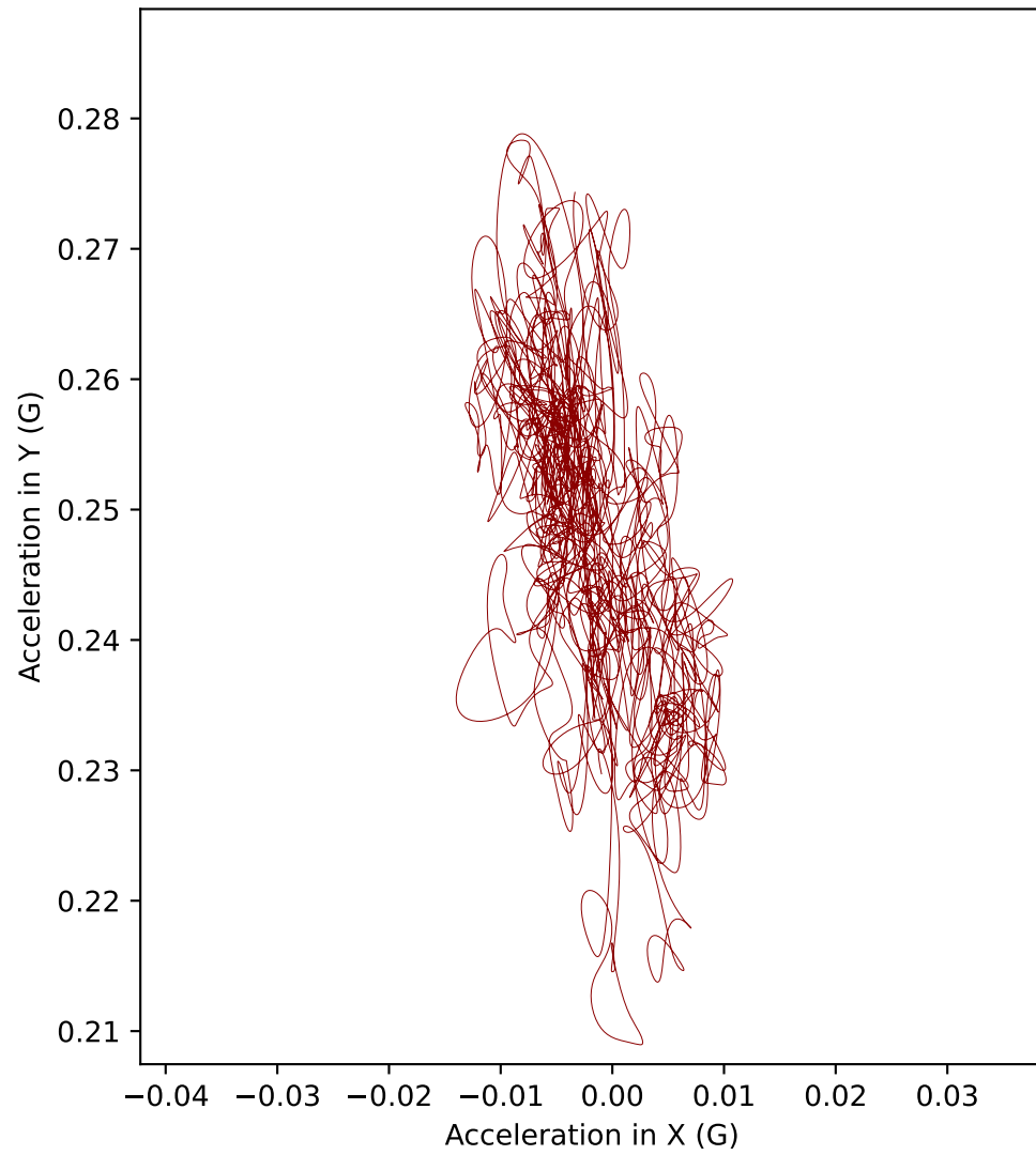
G3 acceleration in XY plane (Top view)
