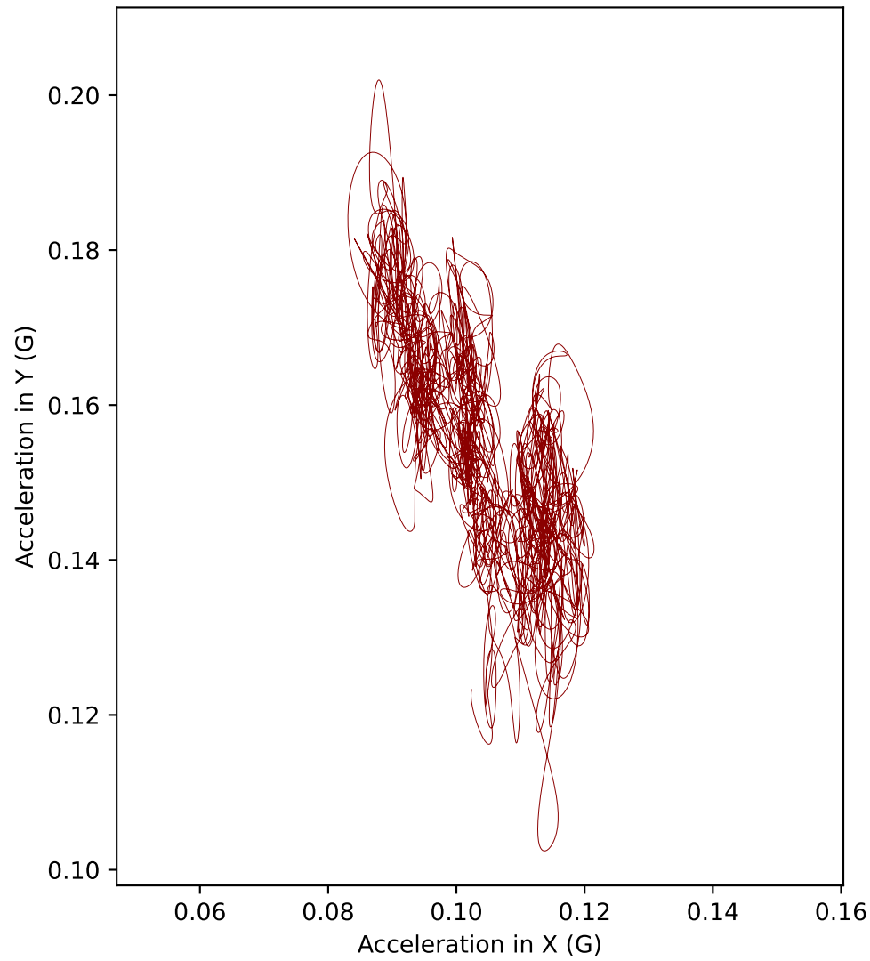
H11 acceleration in XY plane (Top view)
