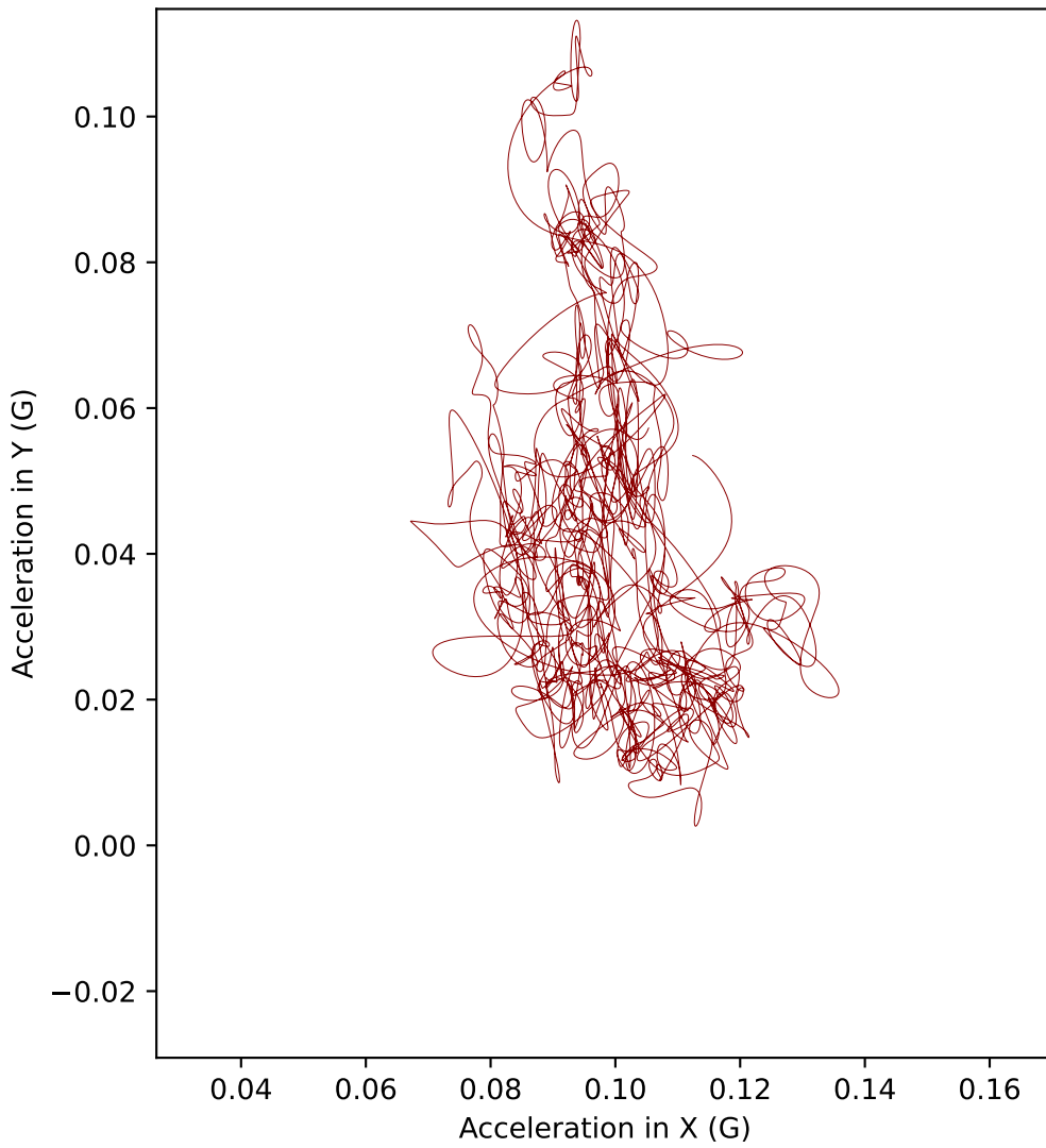
H12 acceleration in XY plane (Top view)
