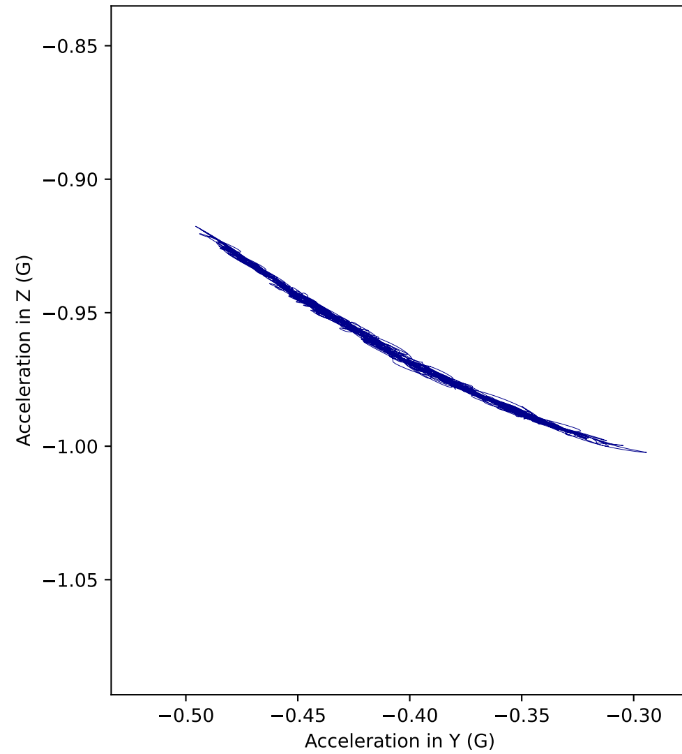
H2 acceleration in YZ plane (Side view)
