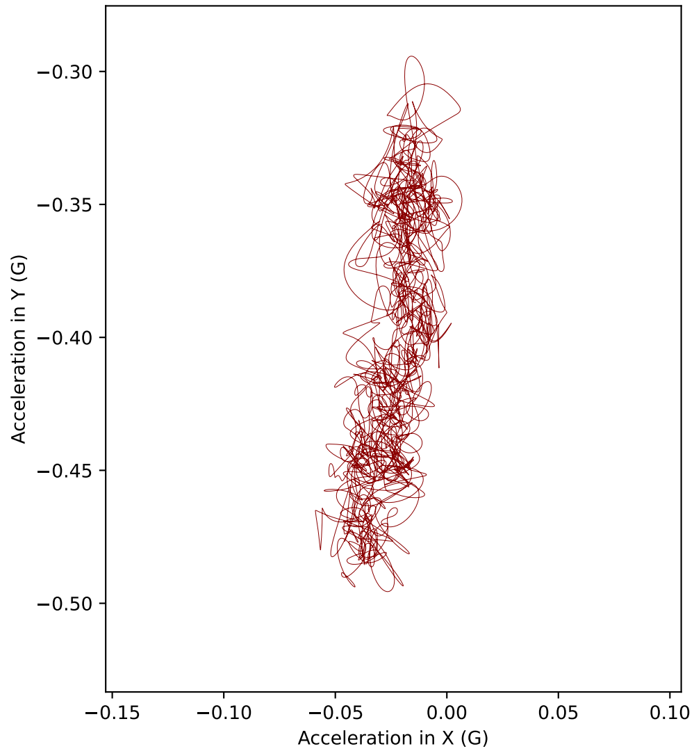
H2 acceleration in XY plane (Top view)
