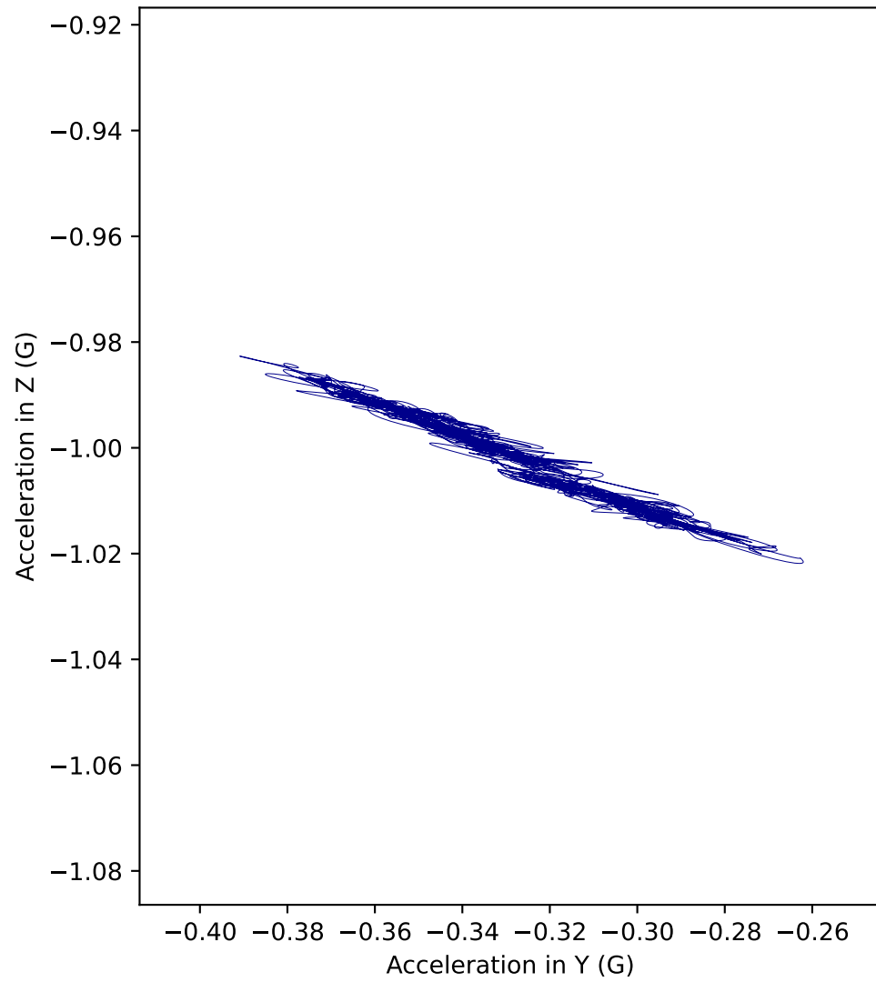
H3 acceleration in YZ plane (Side view)
