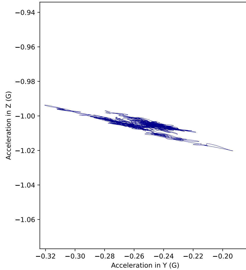
H4 acceleration in YZ plane (Side view)
