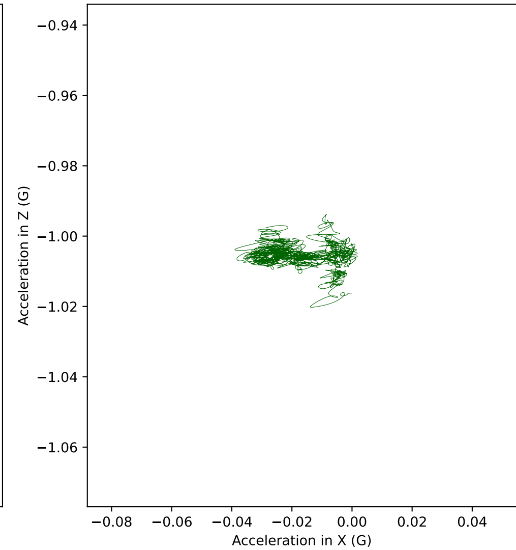
H4 acceleration in XZ plane (Front view)
