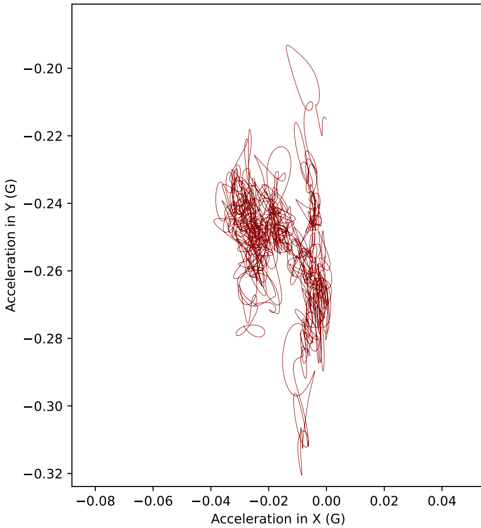
H4 acceleration in XY plane (Top view)
