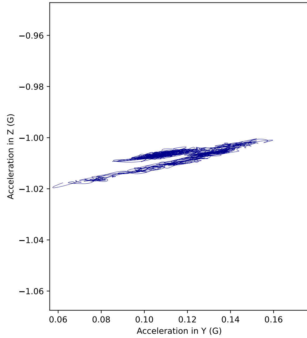
H5 acceleration in YZ plane (Side view)
