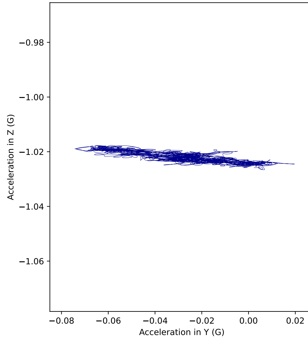
H6 acceleration in YZ plane (Side view)
