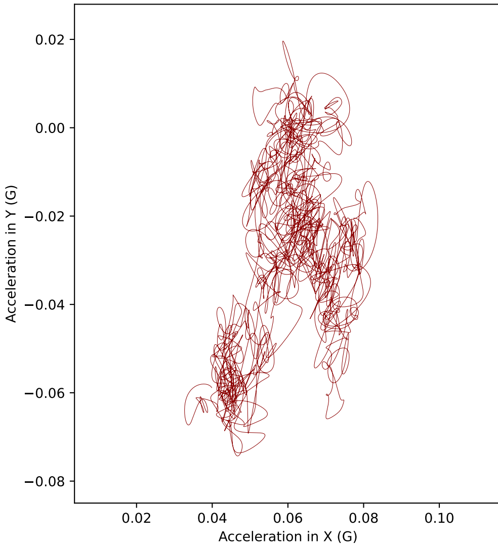
H6 acceleration in XY plane (Top view)
