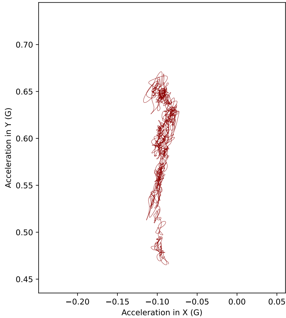
H7 acceleration in XY plane (Top view)
