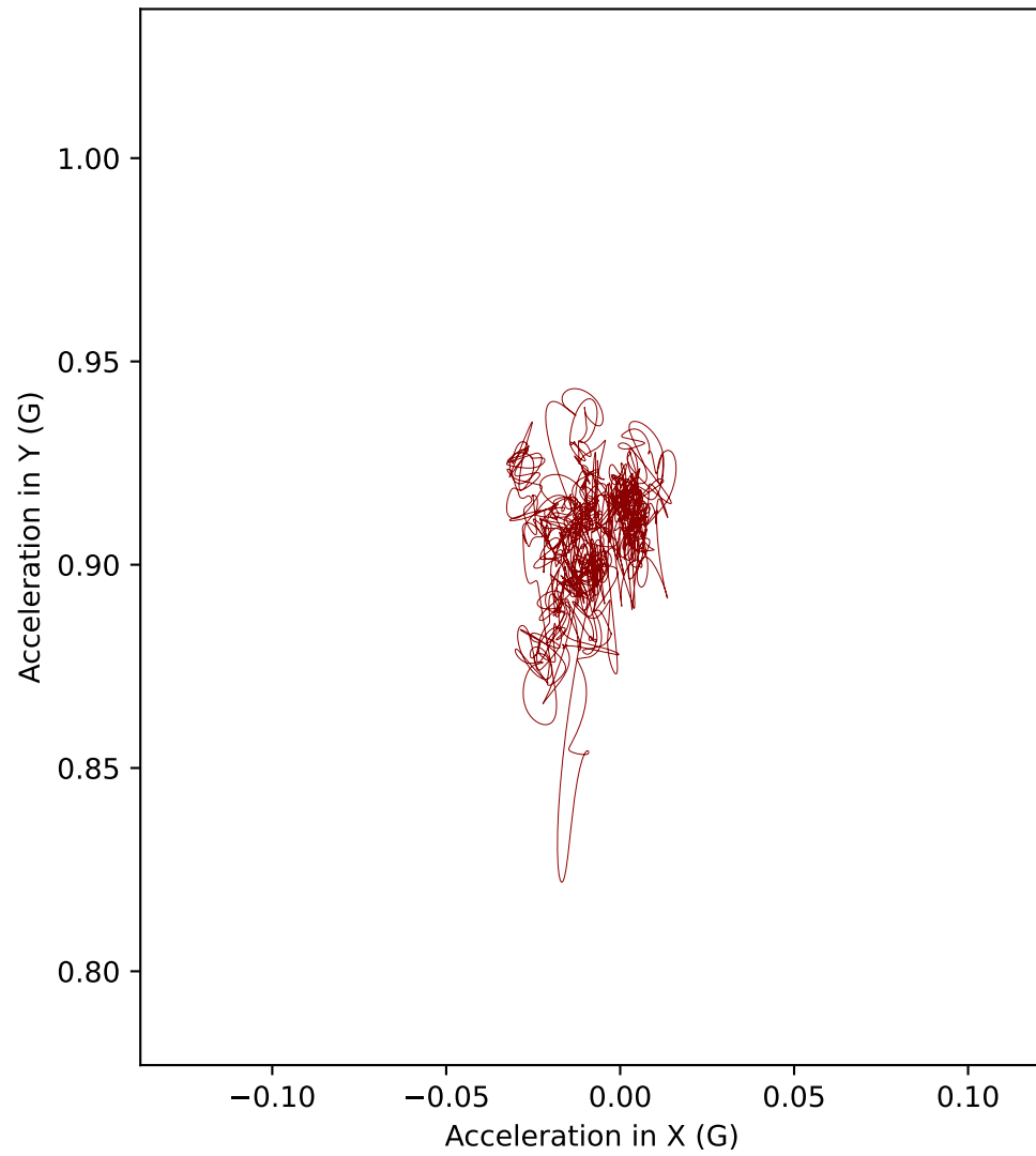
H8 acceleration in XY plane (Top view)
