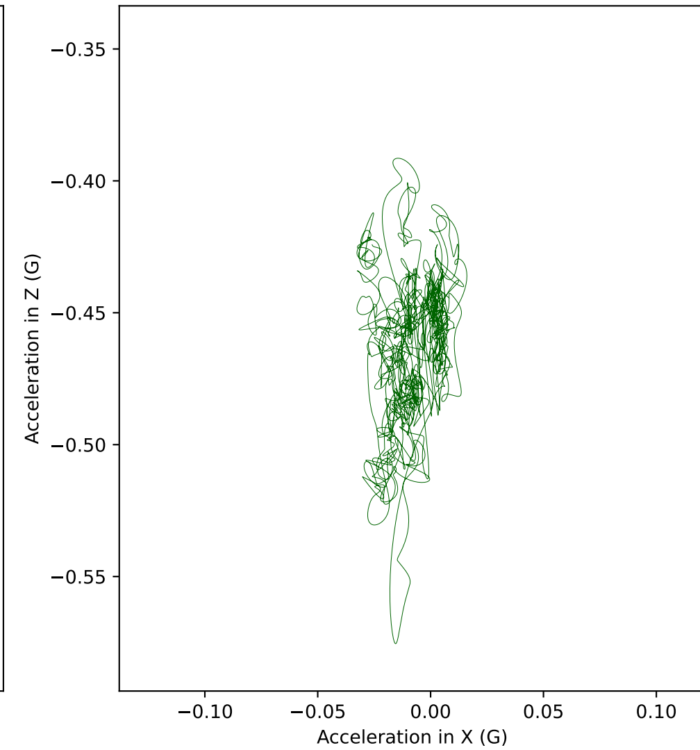
H8 acceleration in XZ plane (Front view)
