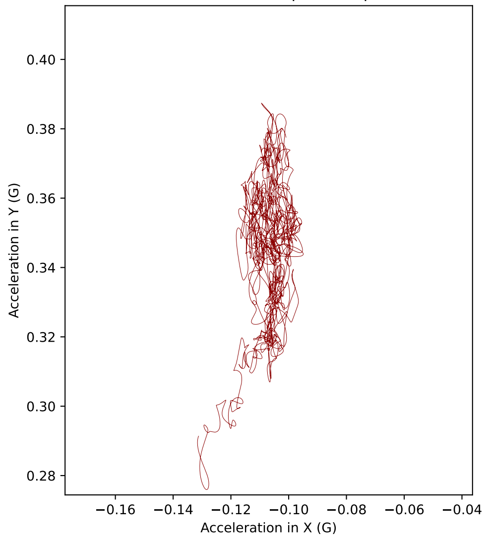
H9 acceleration in XY plane (Top view)
