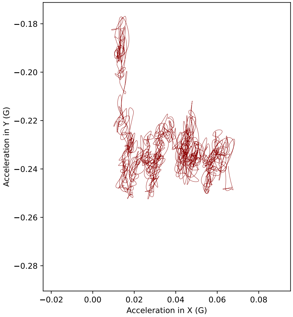
I1 acceleration in XY plane (Top view)
