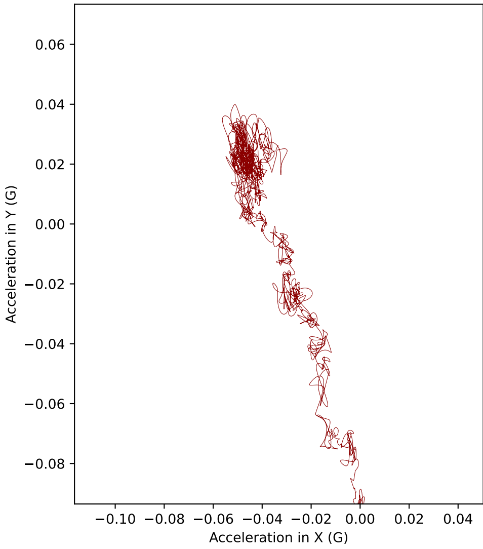
I2 acceleration in XY plane (Top view)
