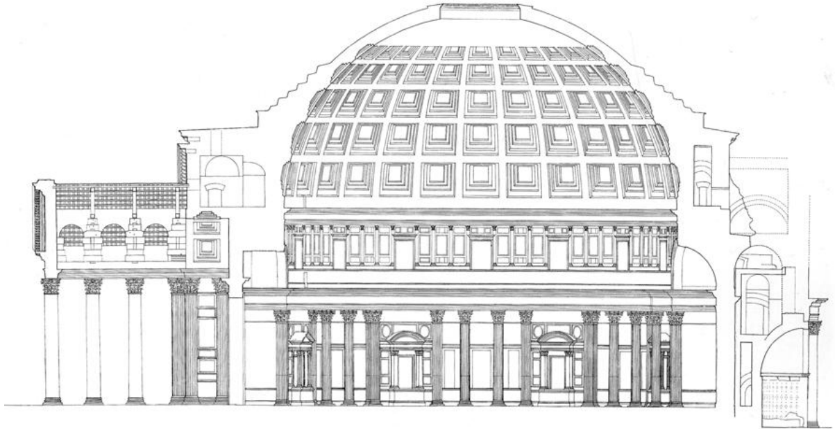
FIG. 105. Pantheon: Longitudinal section along the main axis 1:400.
