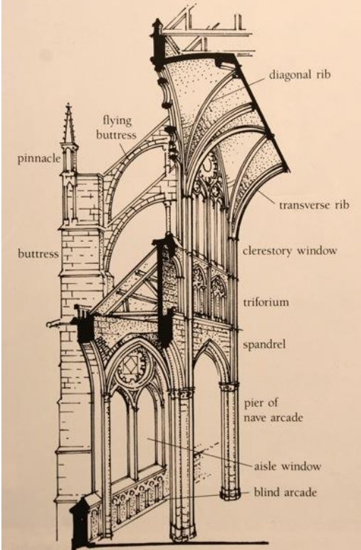
487. Diagrammatic section of Amiens Cathedral with names of the parts in the elevation (after Viollet-le-Duc)
