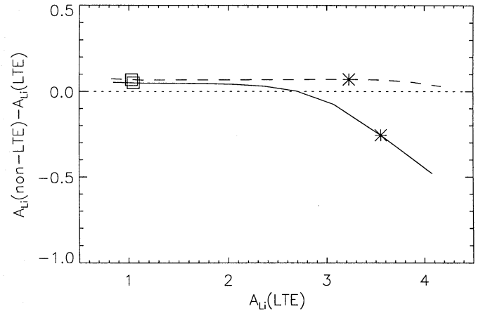
Fig. 10. LTE to non-LTE abundance corrections for solar lithium, respectively for the 670.8 nm resonance line (solid) and the 610.4 nm subordinate line (dashed). The LTE abundance is plotted along the abscissa; this is the value one obtains from our non-LTE computed lines by fitting their equivalent width with LTE line formation using the same atmospheric model. The ordinate measures the corrections that should be added to such LTE estimates to obtain the correct non-LTE abundance. The star on each curve marks the meteoritic lithium abundance A_{\text{Li}} = 3.3 used here for young-sun modeling. LTE abundance analysis of the Li I 670.8 nm line from the young sun would have overestimated its actual lithium abundance by 0.26 dex (a factor 1.8). For lithium-rich stars, the Li I 610.4 nm line is a much better LTE estimator, with an error of only 0.07 dex of opposite sign. The squares mark the present solar abundance A_{\text{Li}} = 1.1
