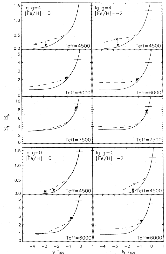
Fig. 12. Planck functions (dashed) and Li I line source functions (solid) at \lambda = 670.8 nm against the logarithm of the continuum optical depth at \lambda = 500 nm. The grid sampling and panel layout are the same as in Fig. 11. Axes, curve coding and marks as in Fig. 5; the marks are again for lithium abundance A_{\text{Li}} = 3.3
