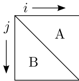
Figure 2: The matrix visualizing the summation.
