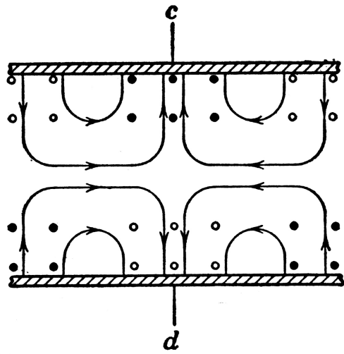
TM_{1,1} Wave
