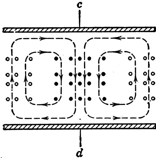
TE_{1,1} Wave
