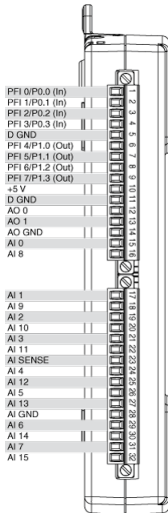
USB-6211/6215 Pinout
