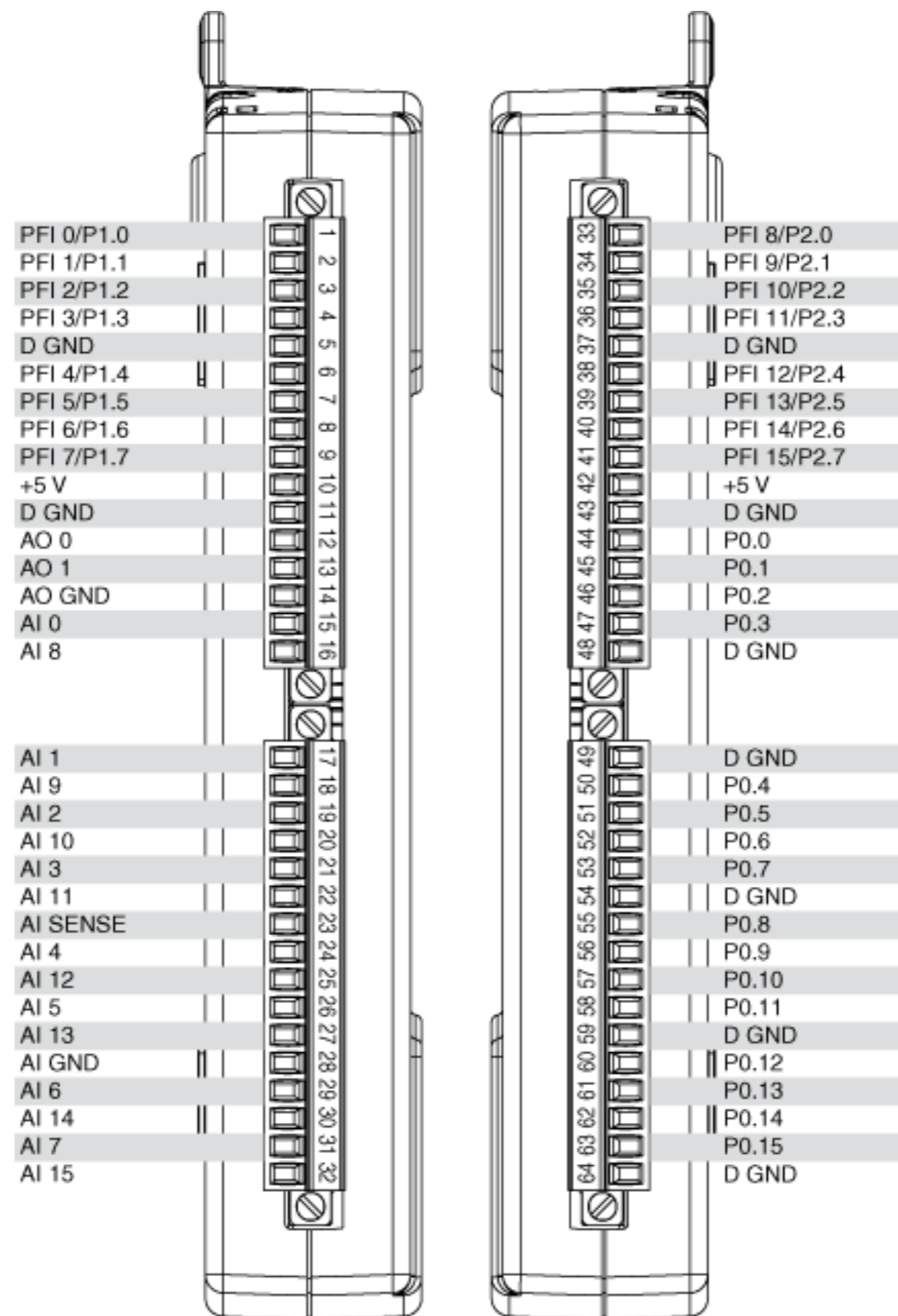
USB-6212/6216 Pinout
