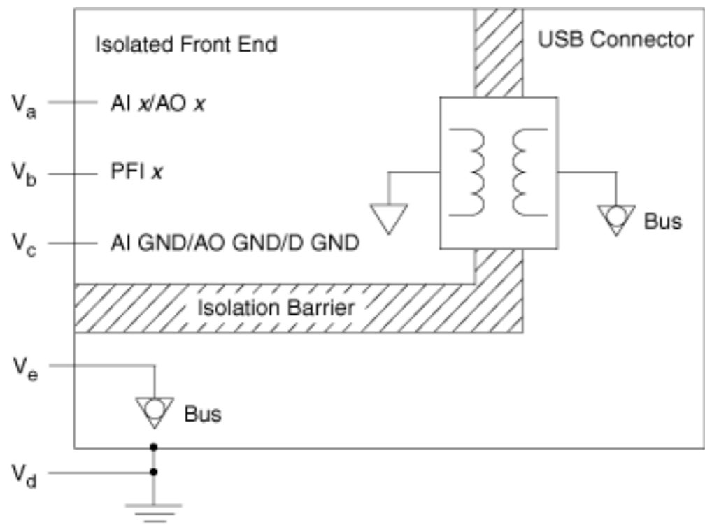
USB-6215/6216/6218 Maximum Working Voltage
