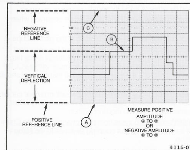
Figure 3-2. Instantaneous voltage measurement.
