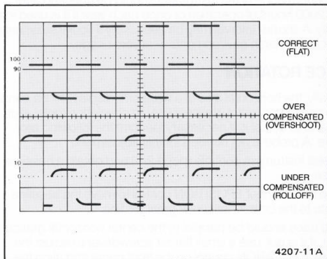
Figure 4-1. Probe compensation.
