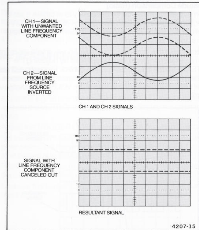
Figure 3-3. Common-mode rejection.
