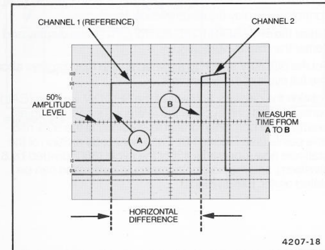
Figure 3-7. Time difference between pulses on time-related signals.
