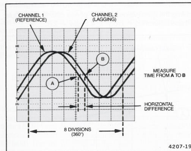
Figure 3-8. Phase difference.
