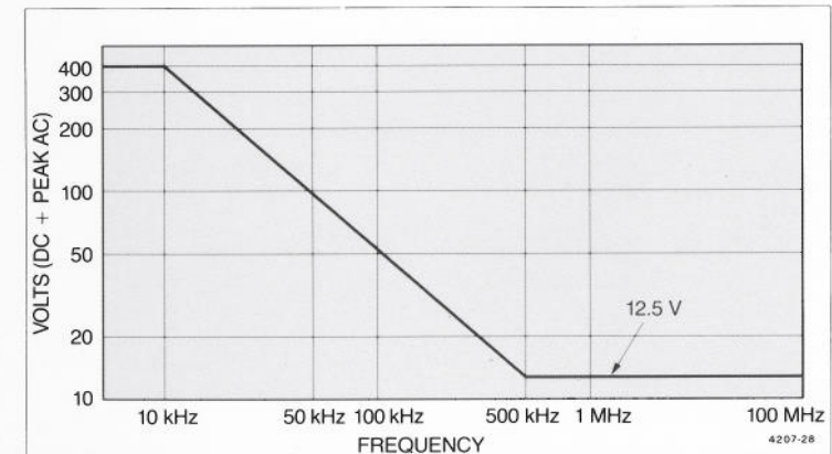
Figure 5-1. Derating curve for CH 1 OR X, CH 2 OR Y, and EXT INPUT connectors.
