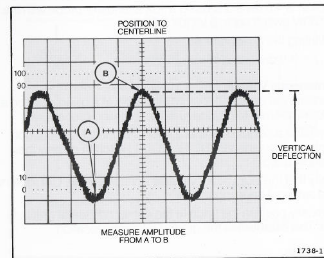
Figure 3-1. Measuring peak-to-peak voltage of a waveform.
