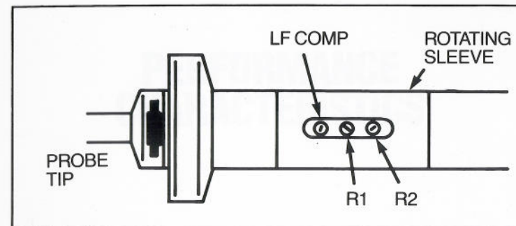
Figure 4-2. Locating the low-frequency compensation adjustment.
