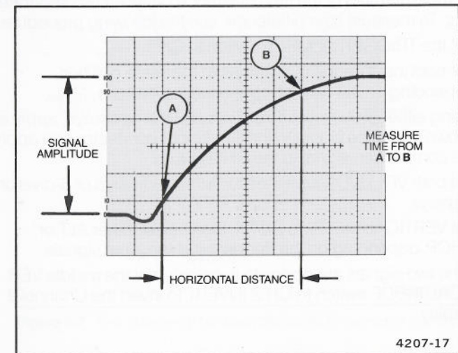
Figure 3-6. Measuring rise time.
