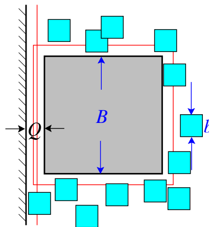
Fig. 6.18 Square pollen grain in fluid of oriented square molecules, next to a wall. The thin lines represents the exclusion region around the pollen grain and away from the wall.
