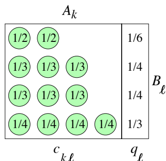
Fig. 5.20 Rational probabilities and conditional entropy. Here the probabilities q_\ell =
