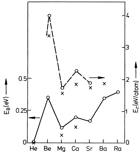
FIG. 13. Well-depths calculated for 1\Sigma_g^+ state of group-IIa dimers (solid line, left scale, Jones, 1979) and cohesive energies of bulk materials (dashed line, right scale, Moruzzi et al. , 1978). Corresponding experimental values (crosses) are given where known (Gschneidner, 1964; Huber and Herzberg, 1979).
