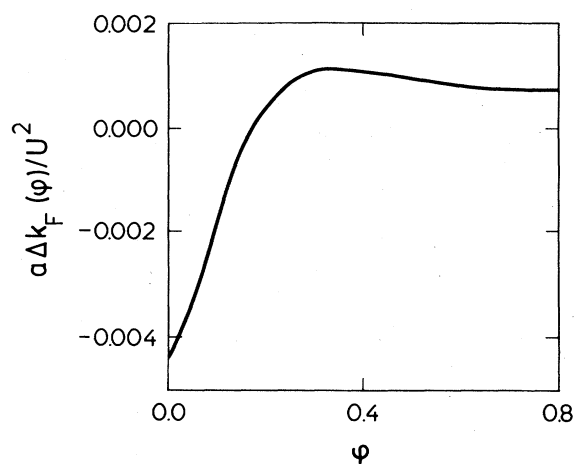
FIG. 38. Deviation \Delta k_F(\varphi) of the Fermi-surface (FS) radius k_F(\varphi) between the quasiparticle FS and Kohn-Sham FS as a function of the angle \varphi for small values of U , where \varphi is the angle to the k_x axis. Because of the symmetry of the Fermi surface, results are shown only for 0 \leq \varphi \leq \pi/4 . The lattice parameter is a and the same energy unit has been used for U , t_1 , and t_2 .
