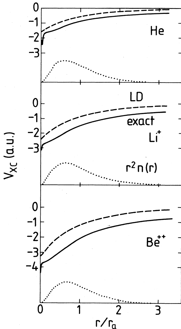
FIG. 5. Exchange-correlation potential V_{\text{xc}} (solid curve) and local-density (LD) value (dashed) for He, \text{Li}^+ , and \text{Be}^{++} . The lengths are in units of atomic radii r_a (0.929, 0.573, and 0.414, a.u., respectively). The radial density is also shown (dotted curve). After Almbladh and Pedroza (1984).
