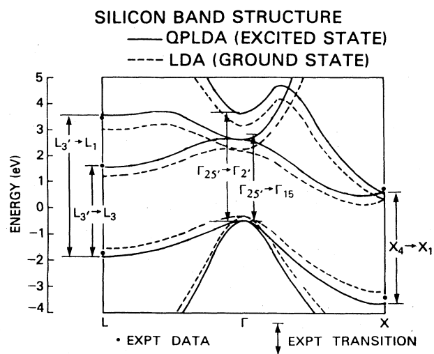
FIG. 39. Quasiparticle (QP) energies of Si (solid lines) according to the calculation of Pickett and Wang (1984) compared with the local-density (LD) energy eigenvalues in the ground-state scheme (dashed lines). Dots and arrows indicate experimental quasiparticle energies and energy differences (Pickett and Wang, 1984).
