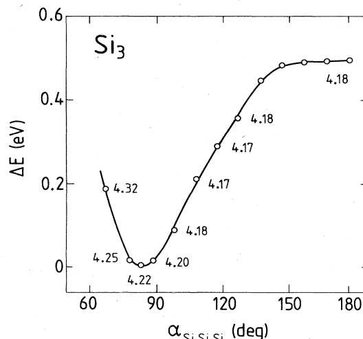
FIG. 18. Energy surfaces for ground state of Si_3 . The optimum bond length for each bond angle \alpha_{SiSiSi} is also shown.
