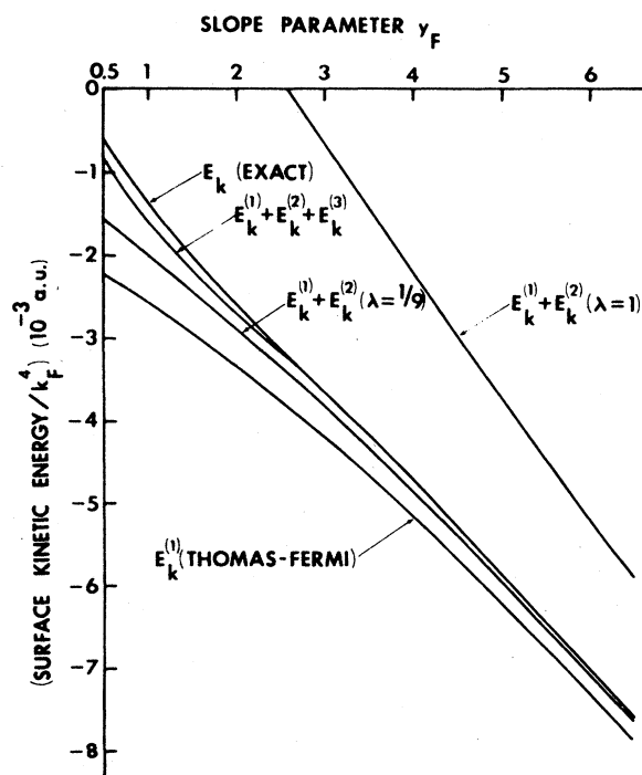
FIG. 3. Surface kinetic energy for the model potential (2.27) as a function of the slope parameter y_F . The exact result [ E_k(\text{EXACT}) ] is compared with the Thomas-Fermi result ( E_k^{(1)} ); with the lowest gradient expansion result ( E_k^{(1)} + E_k^{(2)} ) for both \lambda = \frac{1}{9} and 1; and with the second-order gradient expansion result ( E_k^{(1)} + E_k^{(2)} + E_k^{(3)} ) (Ma and Sahni, 1977).
