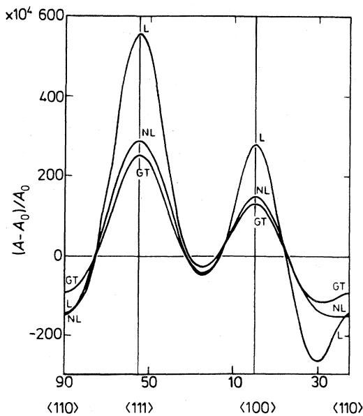
FIG. 40. Extremal Fermi-surface areas for different high-symmetry planes in Cs. The figure compares the local-density eigenvalue results ( L ), the results using the nonlocal potential (6.17) ( NL ), and experimental results ( GT ) (MacDonald, 1980).
