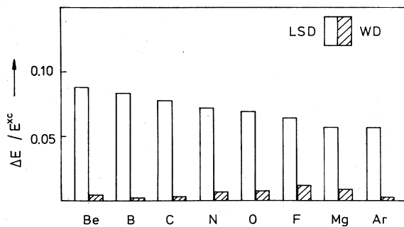
FIG. 30. Error in the total energy of a free atom as a fraction of the exchange-correlation energy in the local spin-density (LSD) and the weighted density (WD) approximations (see Gunnarsson and Jones, 1980a).
