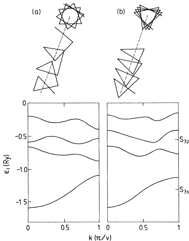
FIG. 24. Geometries (eleven bonds) and electronic band structures of S_\infty : (a) calculated ground-state geometry; (b) at second minimum in Fig. 2. The projections along the helical axis and the atomic eigenvalues are also shown.
