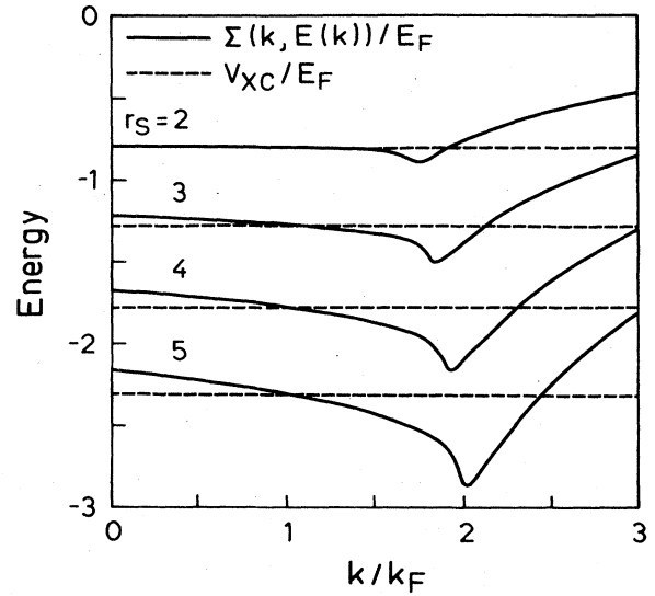
FIG. 35. Self-energy \Sigma (solid curves) and the exchange-correlation potential V_{xc} (dashed curves) for a quasiparticle with momentum k in a homogeneous system with the density n = (\frac{4}{3}\pi r_s^3)^{-1} . The results are expressed in units of the Fermi wave vector k_F and the Fermi energy E_F .
