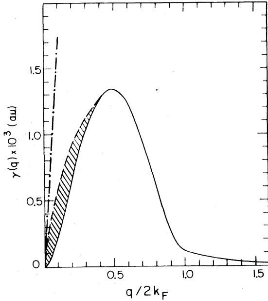
FIG. 32. Wave-vector analysis of the surface energy \Delta E_{xc} = \int d(q/2k_F)\gamma(q) in the random-phase approximation for the infinite barrier model with r_s = 2.07 . The local-density result is given by the solid curve, the k \rightarrow 0 result [Eq. (5.22)] by the dashed-dotted line, and the interpolation by the dashed line. After Langreth and Perdew (1975).
