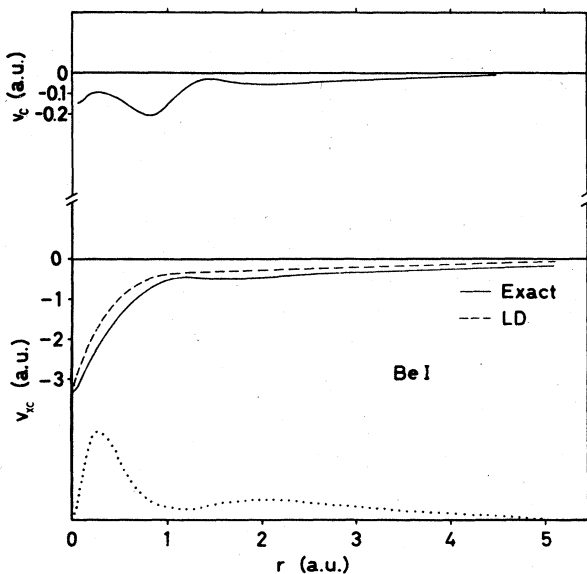
FIG. 36. Accurate exchange-correlation potential V_{xc} compared with the local density (LD) V_{xc} for Be. The dotted line gives the radial density. The upper part of the figure gives the correlation potential (Almbladh and Pedroza, 1984).
