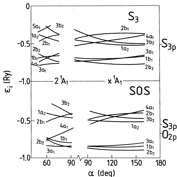
FIG. 21. Self-consistent eigenvalues for the uppermost valence orbitals in S_3 and SOS. For each bond angle \alpha , we show the results for the optimum bond length.
