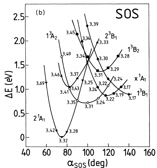
FIG. 20. Energy surfaces for low-lying states of (a) S_3 and (b) SOS . The optimum bond length for each bond angle \alpha is also shown.
