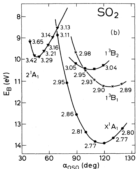
FIG. 19. Energy surfaces for x^1A_1 (circles), 1^3B_1 (crosses), 1^3B_2 (squares), and 2^1A_1 (triangles) states of (a) O_3 and (b) SO_2 . For each bond angle \alpha we show the bond length that optimizes the energy.
