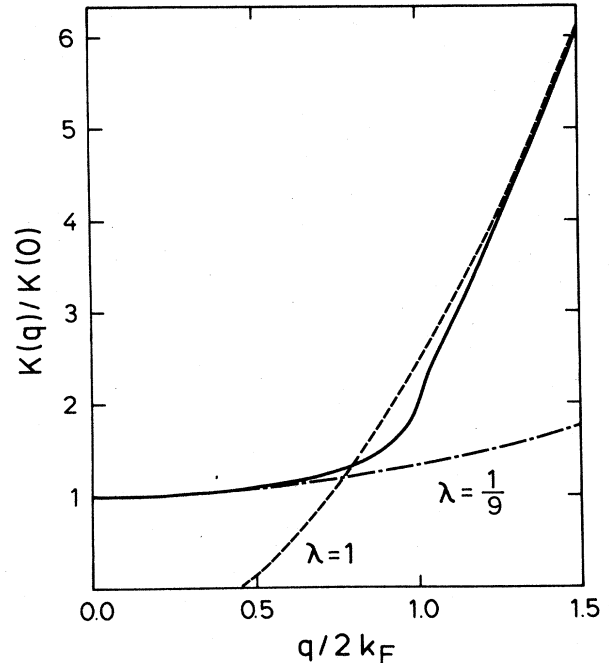
FIG. 2. Function K(q) as a function of q/2k_F (solid curve). The expansion (2.25) is also shown for \lambda = \frac{1}{9} and 1 (dashed curves).
