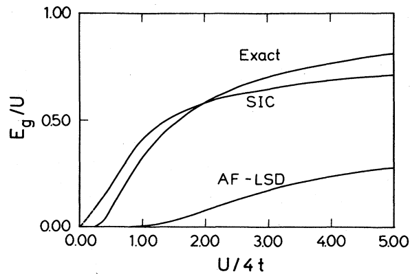
FIG. 31. Band gap E_g for the one-dimensional Hubbard model. The hopping parameter is t and the on-site Coulomb interaction is U . The antiferromagnetic (AF) local spin-density (LSD), the self-interaction corrected (SIC), and the exact results are compared (Svane and Gunnarsson, 1988a).
