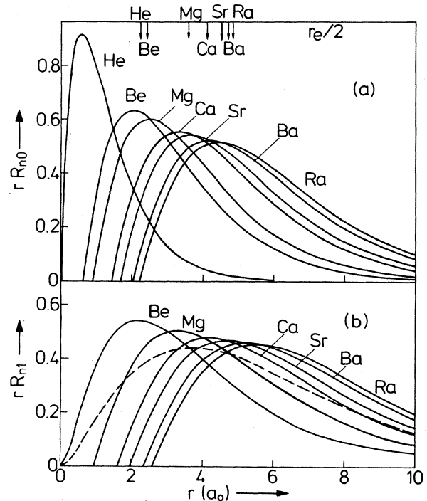
FIG. 14. Tails of valence wave functions for group-IIa atoms: (a) s functions for the 1S(ns^2) states; (b) p functions for the 3P(ns^1np^1) state. The dashed curve is the 2p function of He ( 1s2p ). Also shown (arrows) are distances corresponding to half the calculated equilibrium separation in each dimer (Jones, 1979).
