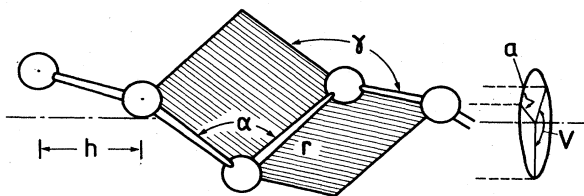
FIG. 22. Structural parameters of a helix with one atom per unit cell.
