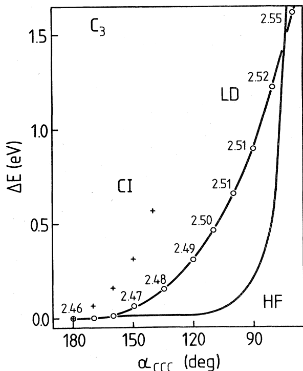
FIG. 17. Energy curves for bending vibration in C_3 . The solid curve shows Hartree-Fock (HF) results for r_{CC} = 2.41 a.u. (Liskow et al. , 1972); the crosses, multiple-reference double-excitation CI (MRD-CI) values for r_{CC} = 2.423 a.u. (Perić-Radić et al. , 1977). Local-density (LD) results are given by circles, and the optimum bond length for each bond angle, \alpha_{CCC} , is also shown (Jones, 1985a).
