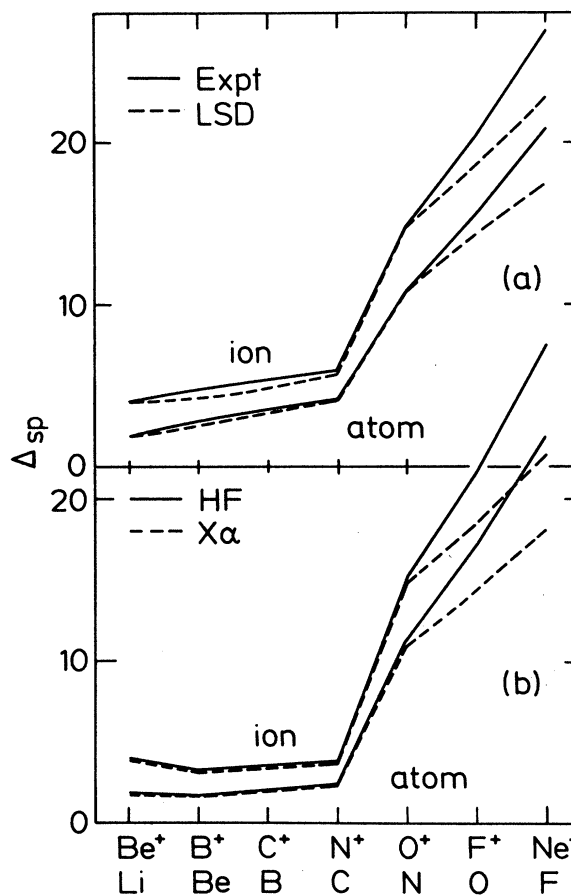
FIG. 9. The sp transfer energies \Delta_{sp} for the first-row atoms and ions: (a) experimental and local spin-density (LSD) results; (b) Hartree-Fock (HF) and X\alpha results. The energies are in eV.
