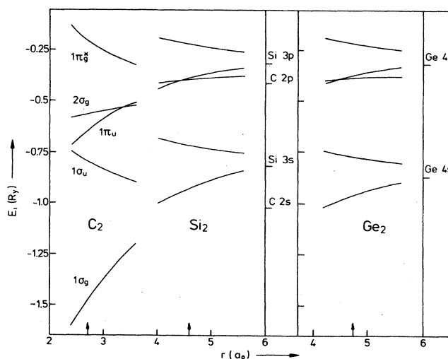
FIG. 16. Self-consistent eigenvalues for ^3\Sigma_g^- state of \text{C}_2 , \text{Si}_2 , and \text{Ge}_2 . Also shown are the valence eigenvalues for the isolated atoms. The arrows denote the calculated equilibrium separations in each case.
