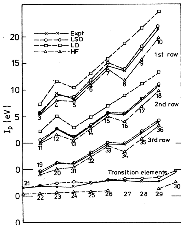
FIG. 8. First ionization energy of atoms in the local-density (LD), local spin-density (LSD), and Hartree-Fock (HF) approximations compared with experiment. The numbers show the atomic numbers of the atoms considered. For reasons of clarity, the zero of energy is shifted by 5, 10, and 15 eV for the second row, the third row, and the transition-element row, respectively. The LD results for the first and second rows are increased by an additional 2 eV.
