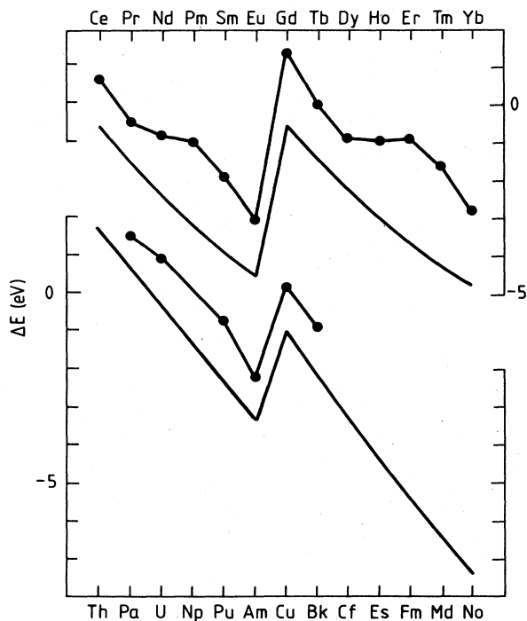
FIG. 11. The df transfer energies \Delta_{df}[E(f^{n-3}d^2) - E(f^{n-2}s^2)] for rare-earth and actinide atoms (Glötzel, 1980). The calculations (solid lines) are for spherically averaged densities.
