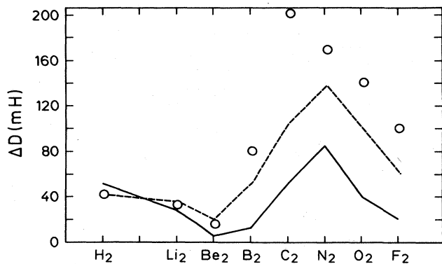
FIG. 34. Correlation energy contribution to the dissociation energy of some dimers. The local spin-density (solid line), the Langreth-Mehl (dashed line), and the empirical (circles) results are shown (after Savin et al. , 1986).
