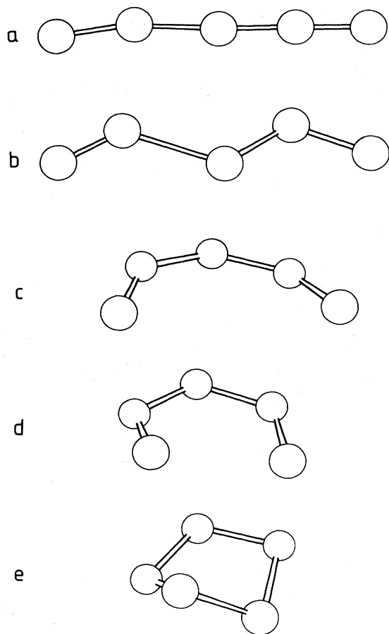
FIG. 26. Deformation of \text{Se}_5 linear chain to the calculated ground-state structure (Hohl et al. , 1987b).
