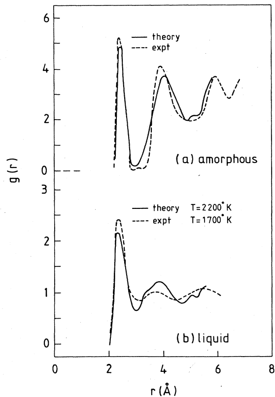
FIG. 25. Pair correlation function g(r) for (a) amorphous and (b) liquid Si (after Car and Parrinello, 1987).
