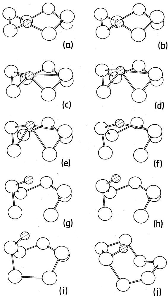
FIG. 27. Structural changes in \text{S}_7\text{O} at T=2000 K. (a)–(i) Evolution of the "ring" structure into the "intermediate" structure (Hohl et al. , 1989). The interval between each frame is 150 time steps, each of 1.7 \times 10^{-16} sec. (j) The ground-state structure from the same perspective.
