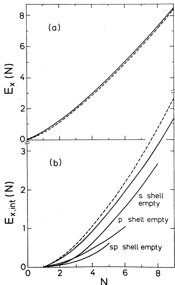
FIG. 28. Exchange energies in model described in text. (a) E_x^{X\alpha} (dashed curve) and E_x^{HF} (solid curve) as a function of the number N of electrons (in units of -G_0 ); (b) the interelectronic exchange E_{x,\text{int}} for the X\alpha and Hartree-Fock (HF) approximations. In the HF approximation we show the dependence for different schemes of occupying the orbitals.
