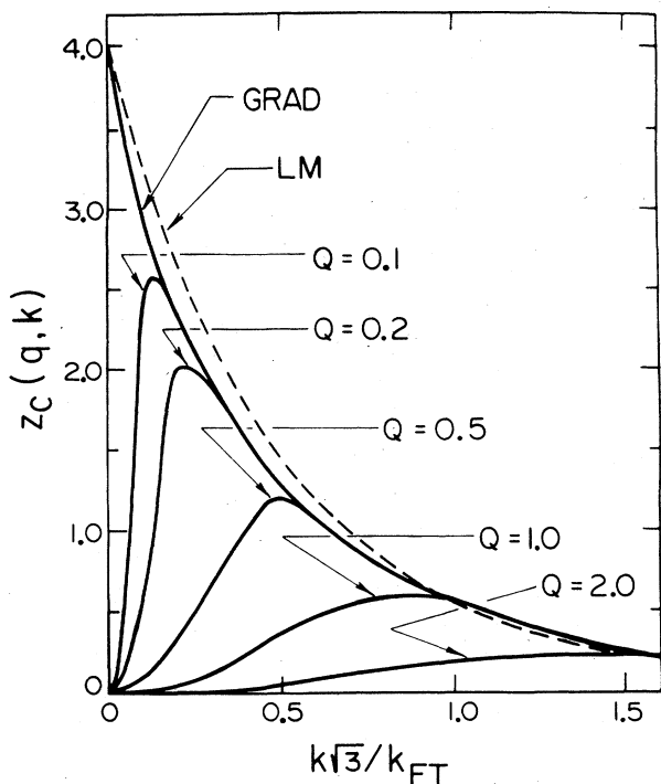
FIG. 33. Wave-vector decomposition of \bar{Z}_c(k_F, Q) [Eq. (5.33)] for the almost homogeneous density (5.28) and (5.29) for different values of Q . The unit of Q is k_{FT}/\sqrt{3} . The curve labeled GRAD shows the corresponding result for the gradient expansion; the dashed curve (LM) shows the result for the interpolation formula (5.37). The LM (Langreth-Mehl) approximation consists of truncating the dashed curve at k = k_c \sim Q .
