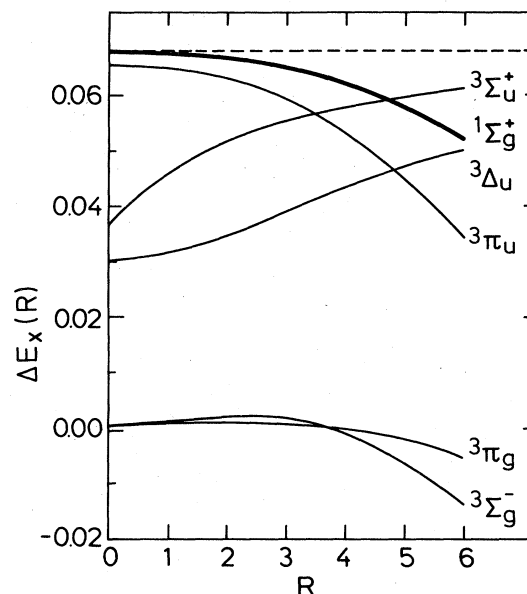
FIG. 29. Difference \Delta E_x(R) between the exchange energies in the X\alpha and Hartree-Fock approximations as a function of the internuclear separation R for different states of the \text{Li}_2 molecule. For the ground state the equilibrium separation is R = 5 a.u. The dashed curve shows the result for two free Li atoms. All energies are in Ry.
