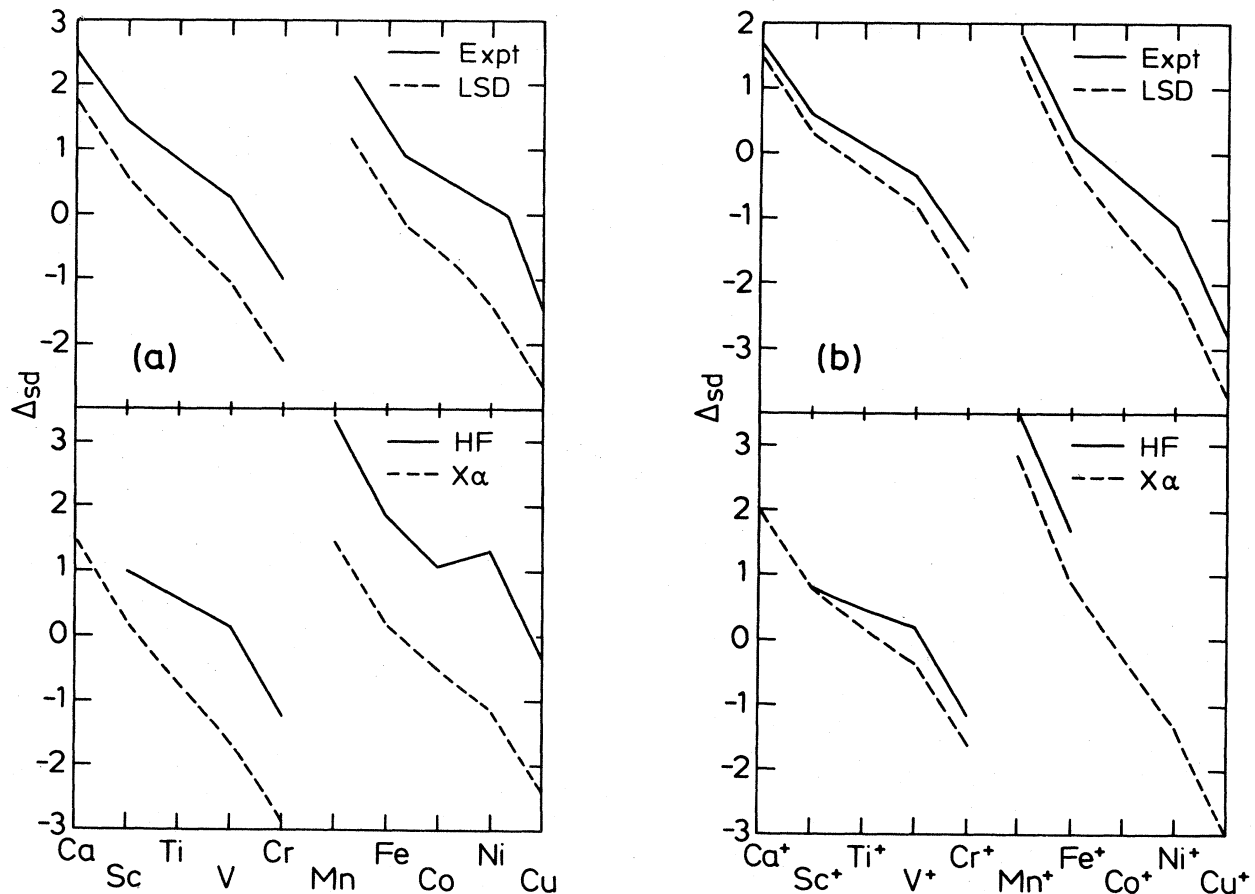
FIG. 10. The sd transfer energies \Delta_{sd} for (a) 3d atoms and (b) 3d ions. In the upper panels, local spin-density (LSD) and experiment are compared; in the lower panels, X\alpha and Hartree-Fock (HF) are compared.
