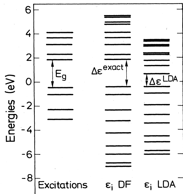
FIG. 37. Eigenvalue spectrum ( \epsilon_i ) and the corresponding excitation energies for a semiconductor chain with nine atoms. E_g shows the exact band gap (Gunnarsson and Schönhammer, 1986).
