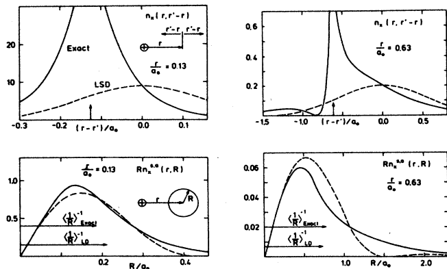
FIG. 7. Exact (solid line) and approximate (dashed line) exchange hole n_x(r, r'-r) [Eq. (3.10)] for a spin-up electron in a nitrogen atom for r=0.13 and 0.63 a.u. The top figure shows the hole along a line through the nucleus and the electron. The arrow indicates the nuclear position and r-r'=0 gives the electron position. The exact hole has a large weight at the nucleus, while the approximate hole is centered at the electron. The lower figure shows the spherical average of the hole around the electron. The area under the curve is proportional to the exchange energy. The figure also shows the value of \langle 1/R \rangle , defined in Eq. (3.13).
