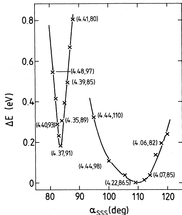
FIG. 23. Total energy surfaces (relative to ground-state minimum) of sulfur helix as a function of bond angle \alpha_{SS} . Values of (r_{SS}, \gamma_{SSSS}) are also shown.
