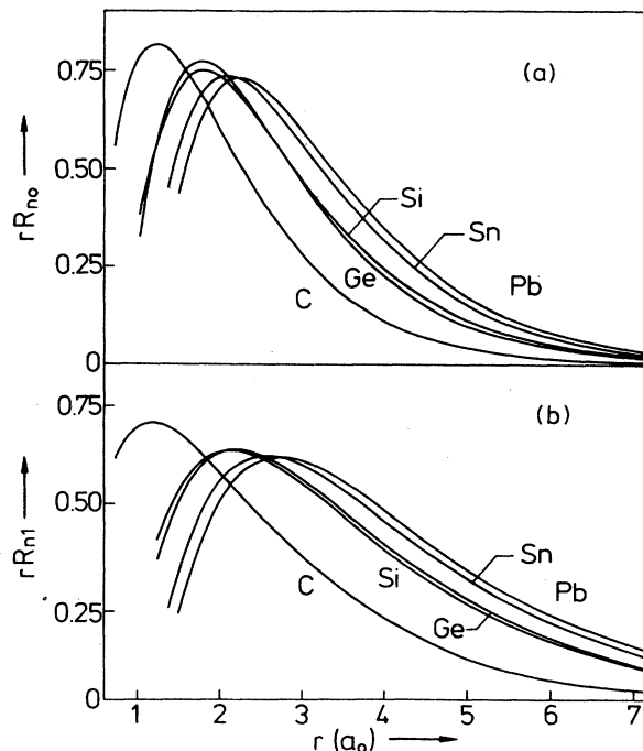
FIG. 15. Radial valence functions for group-IVa atoms: (a) s functions; (b) p functions.
